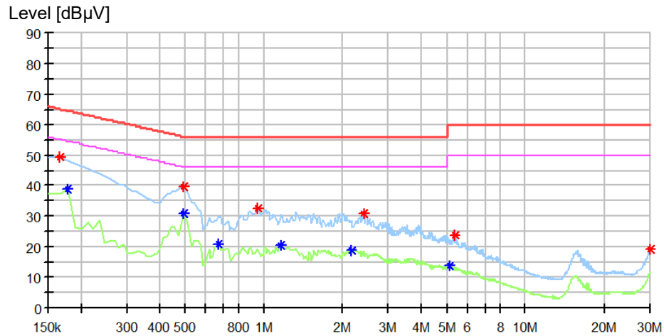
Figure 4: Spectral Diagrams, Conducted Emission, 150 kHz – 30 MHz, Mode 2, N Line
