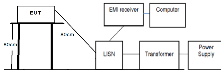
(Conducted emission)
