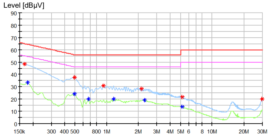
Figure 2: Spectral Diagrams, Conducted Emission, 150 kHz – 30 MHz, Mode 1, N Line
