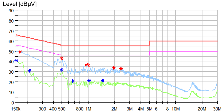
Figure 3: Spectral Diagrams, Conducted Emission, 150 kHz – 30 MHz, Mode 2, L Line
