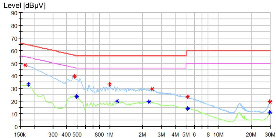
Figure 1: Spectral Diagrams, Conducted Emission, 150 kHz – 30 MHz, Mode 1, L Line
