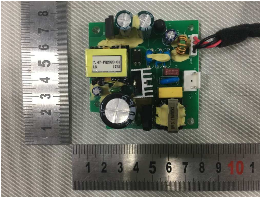
Picture 7- Power supply board
