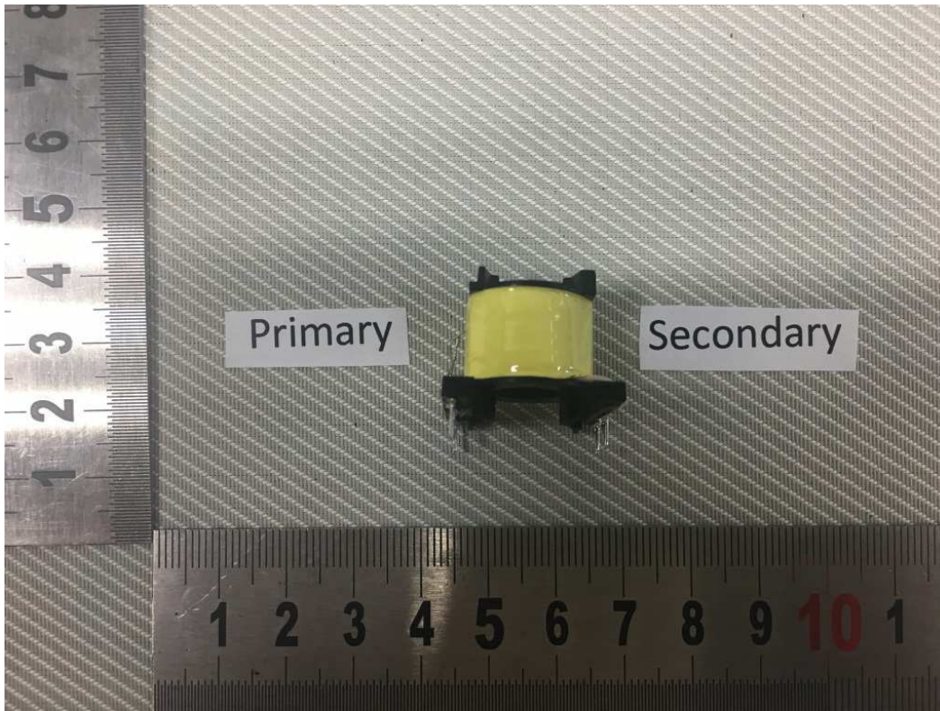
Picture 21- Transformer
