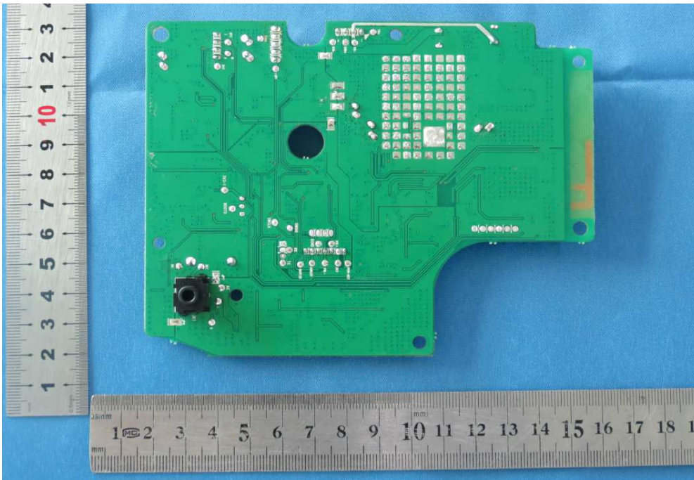
Picture 5- Mainboard
