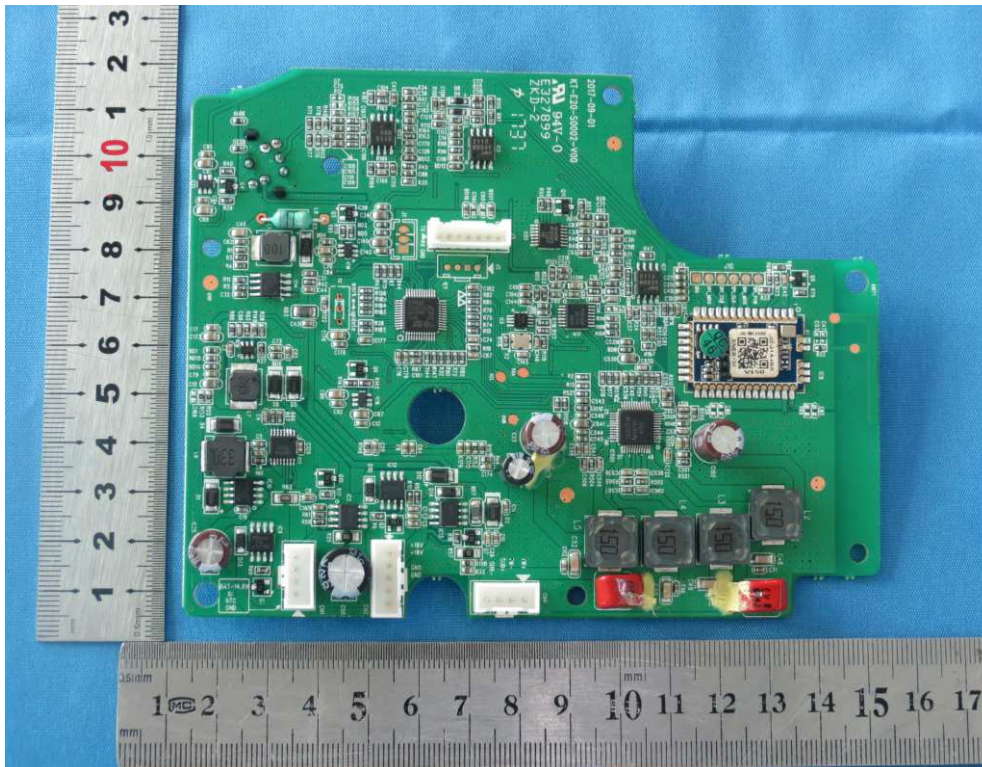
Picture 4- BT Module
