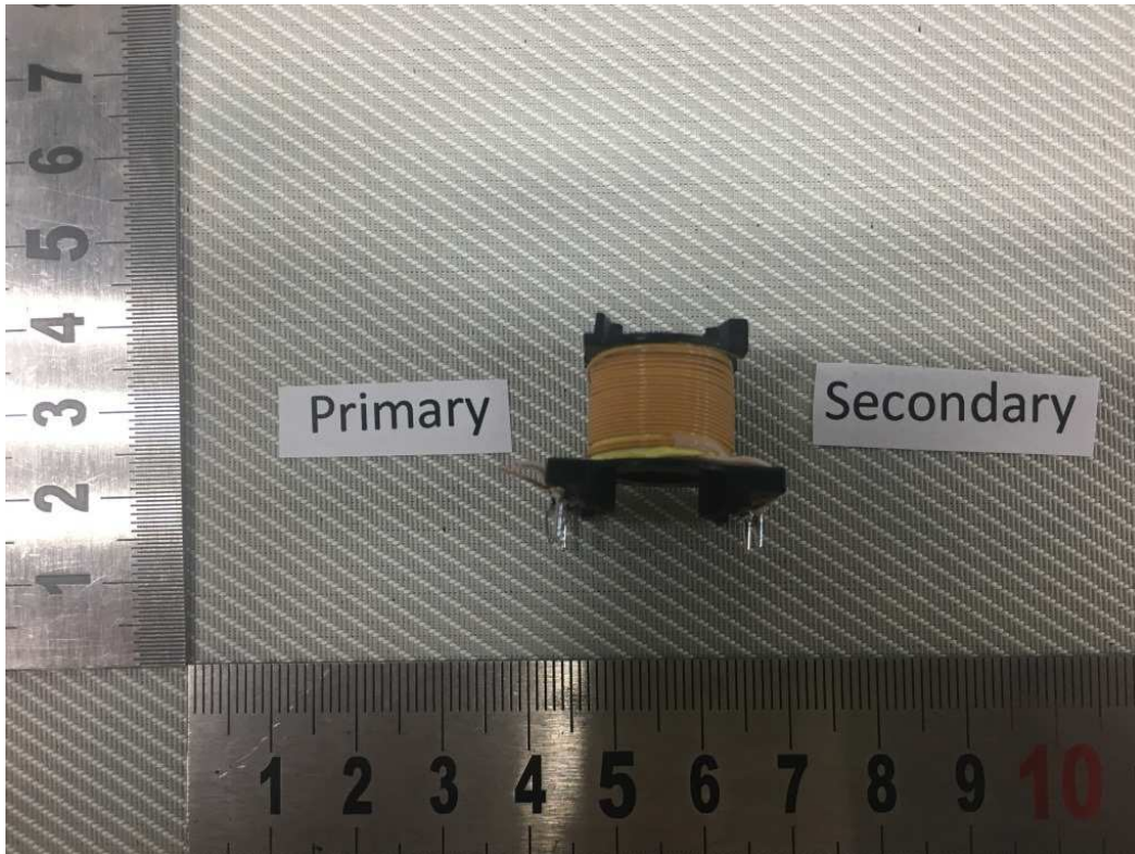
Picture 22- Transformer
