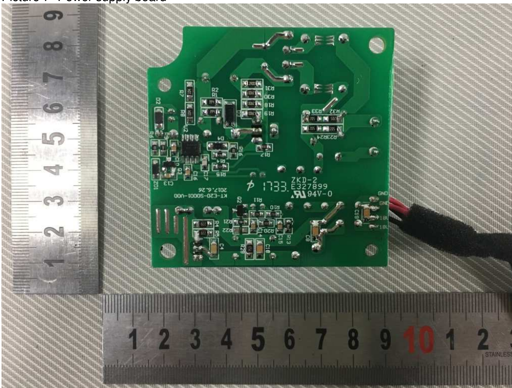
Picture 8- Power supply board
