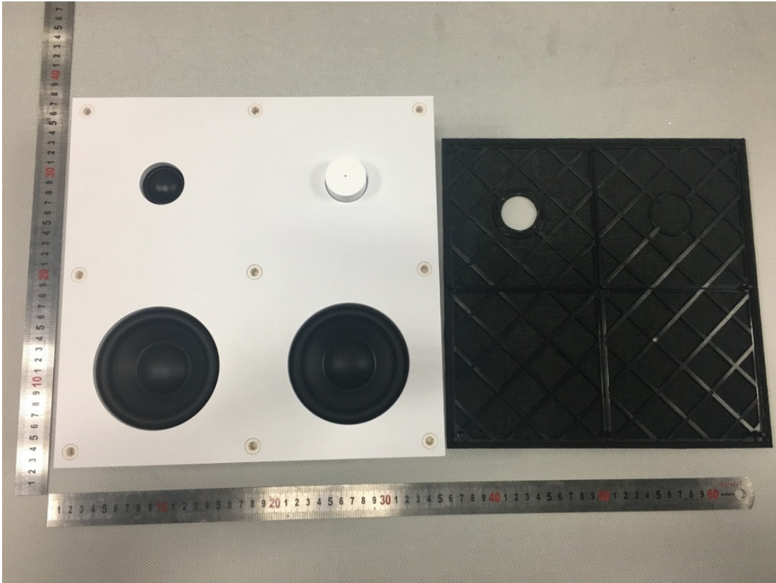
Picture 13- Front view after remove cover (white)
