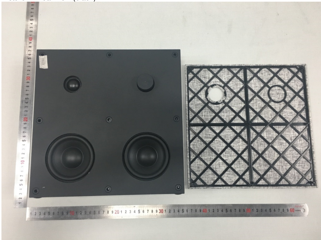
Picture 8- Front view after remove cover (black)
