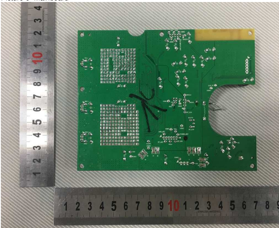
Picture 7- Mainboard
