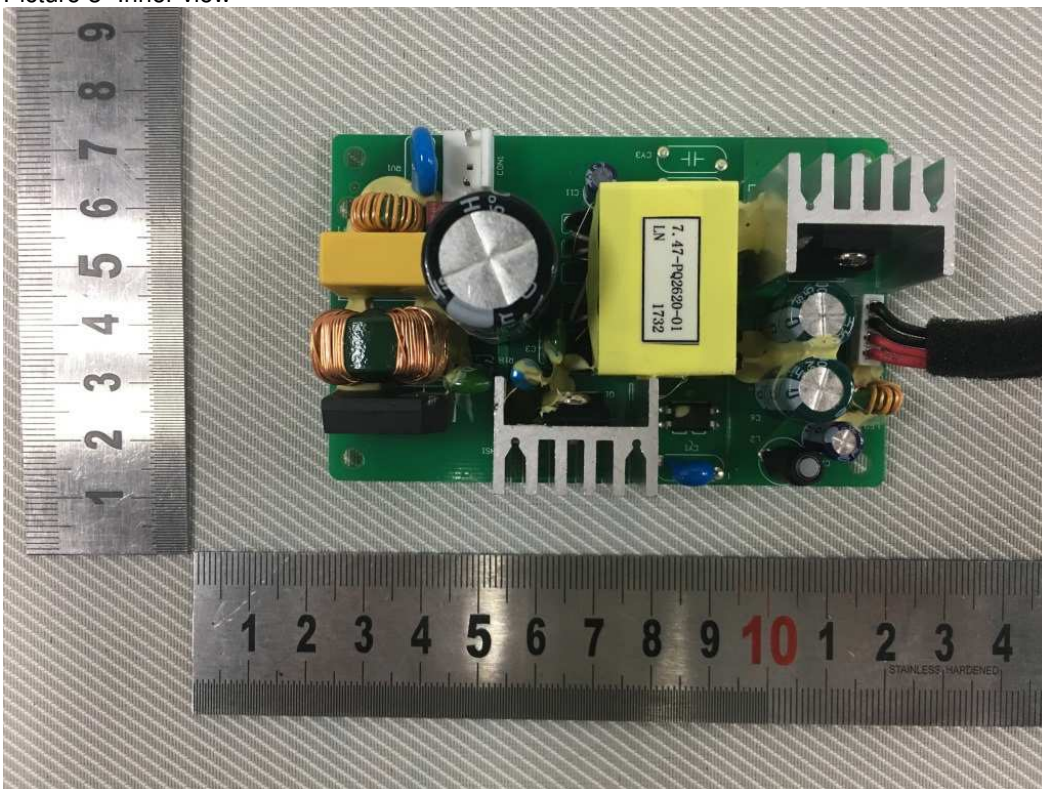
Picture 4- Power supply board
