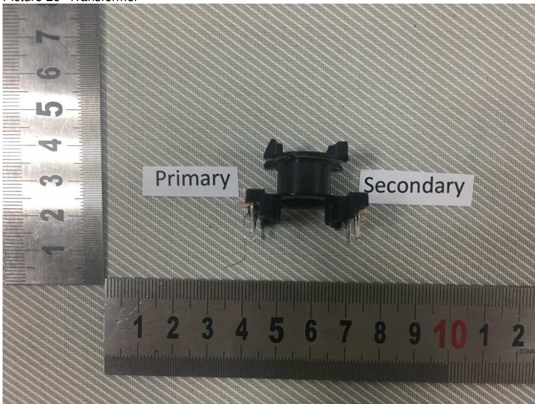
Picture 27- Transformer
