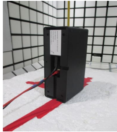
VERTICAL – ORIENTATION
