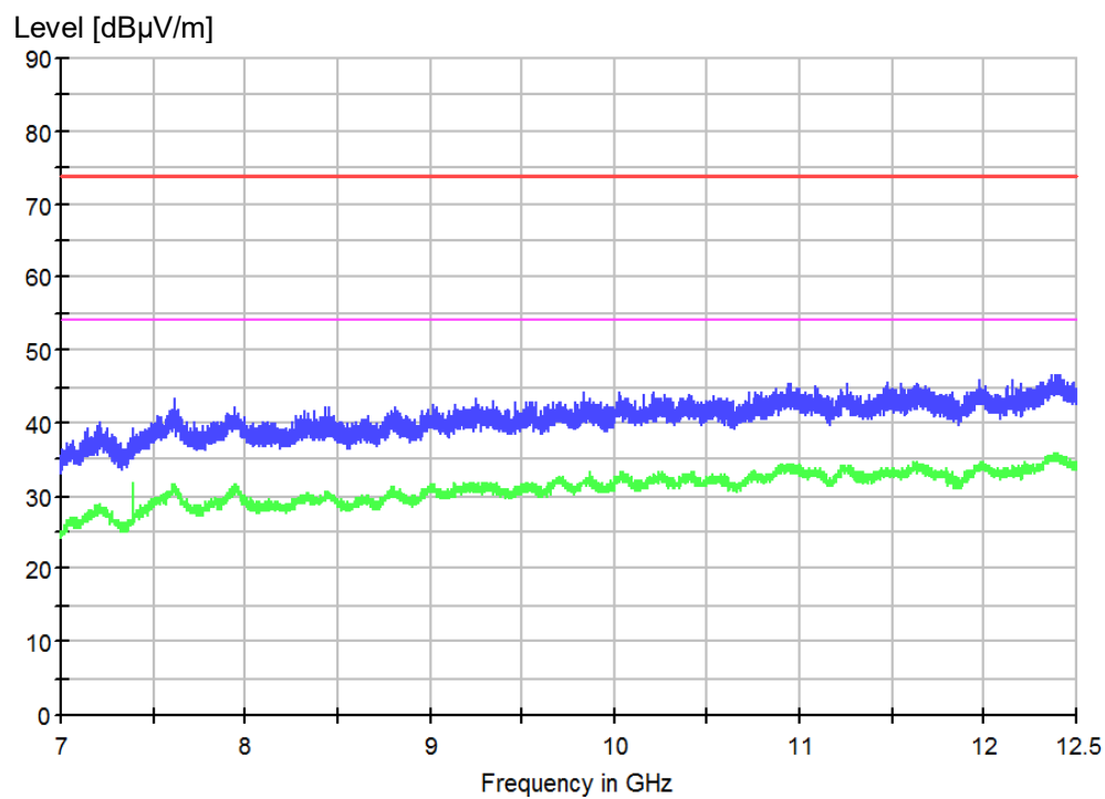
Figure 23: Spectral Diagrams and measurement results, 7 GHz-12.5 GHz, horizontal polarization for mode 1
