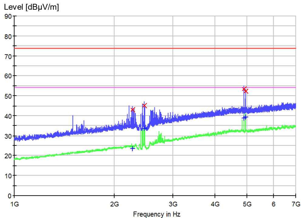
Figure 22: Spectral Diagrams and measurement results, 1 GHz-7 GHz, vertical polarization for mode 4
