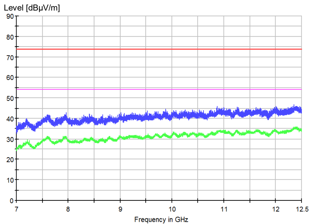
Figure 27: Spectral Diagrams and measurement results, 7 GHz-12.5 GHz, horizontal polarization for mode 3
