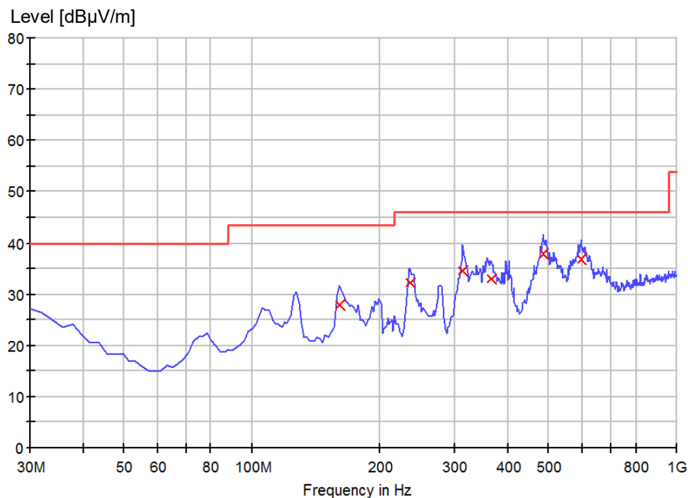
Figure 8: Spectral Diagrams and measurement results, vertical polarization (30 MHz to 1 GHz) for mode 1
