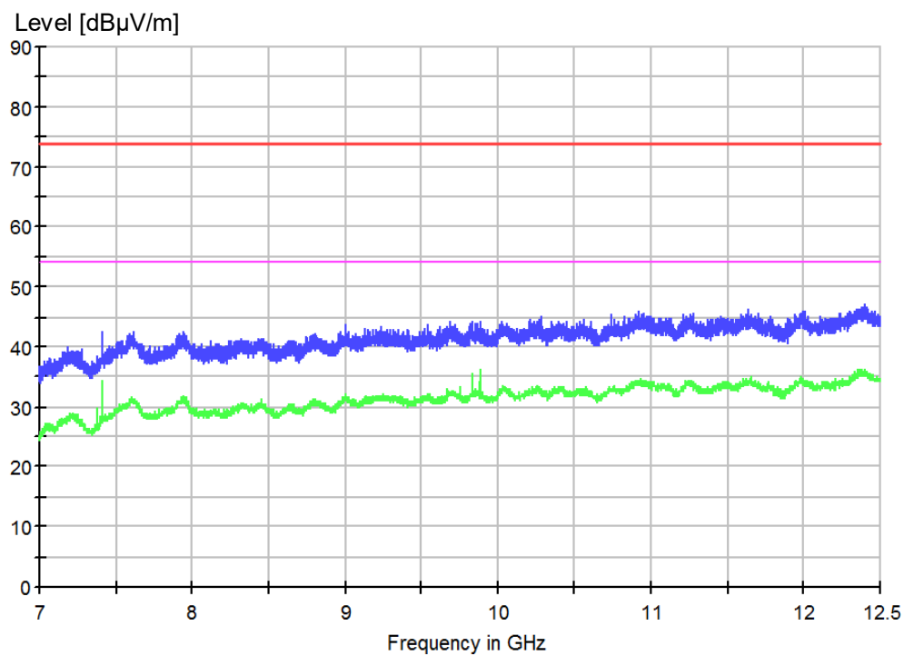
Figure 30: Spectral Diagrams and measurement results, 7 GHz-12.5 GHz, vertical polarization for mode 4
