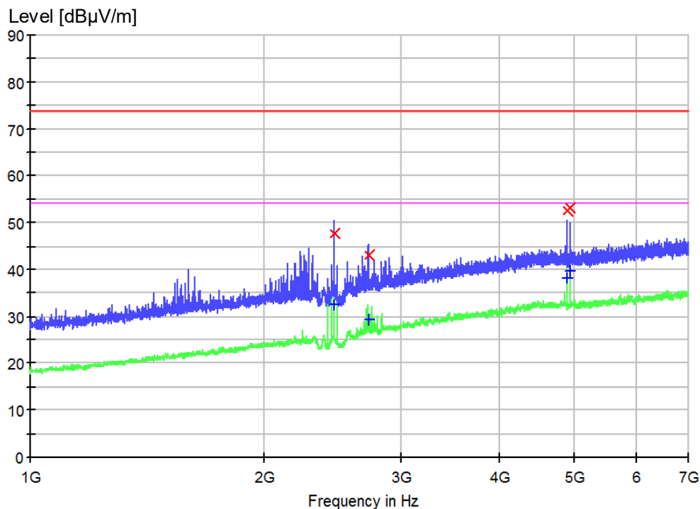
Figure 20: Spectral Diagrams and measurement results, 1 GHz-7 GHz, vertical polarization for mode 3
