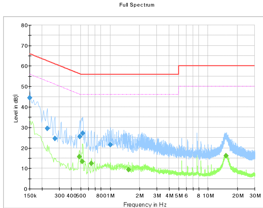
Figure 20: Conducted Emission, TM5, N
