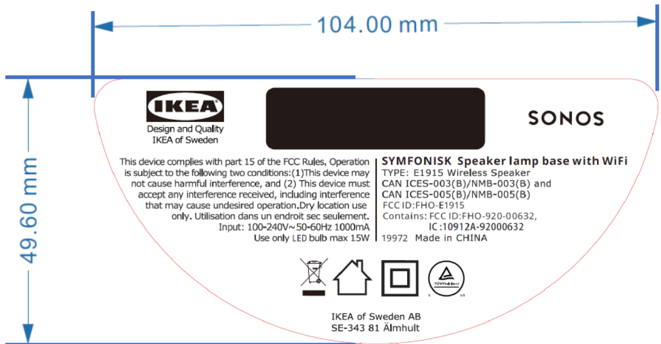
(fig. 5) Bottom view showing label content (Mass Production label – “MP1”)
