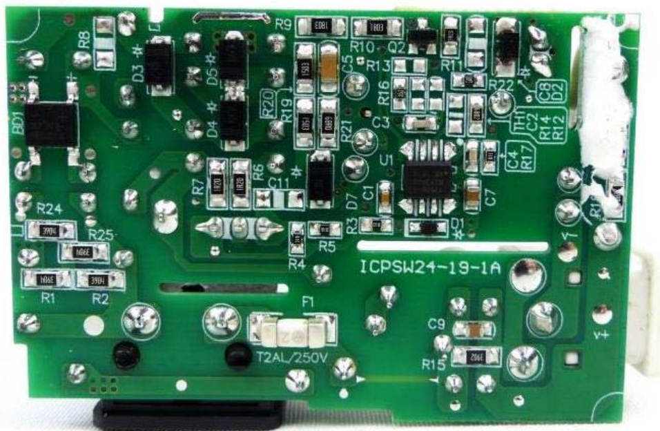
Rear view of adapter PCB (ICPSW24-19-1A)
