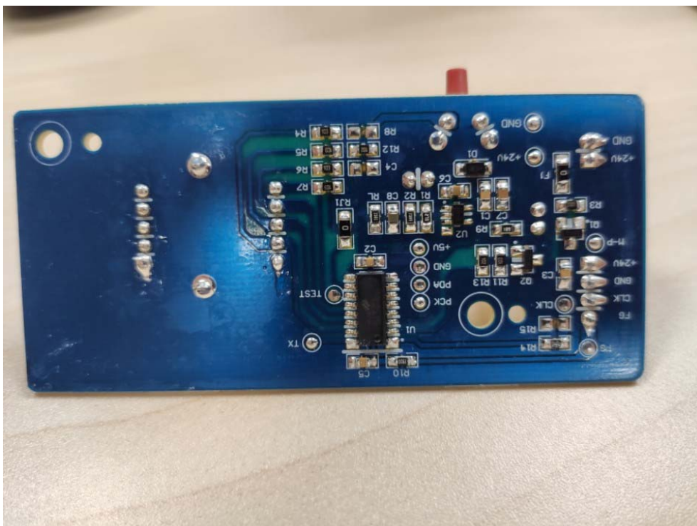
Control board PCB view
