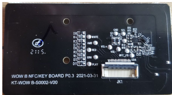
(fig. 11) LED Button NFC board (rear)
