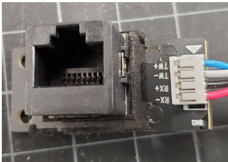
(fig. 4) RJ45 connector board (component side)
