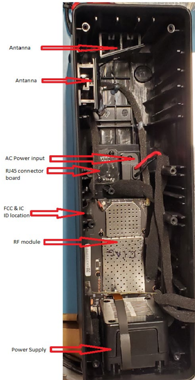
(fig. 7) Internal photo.
