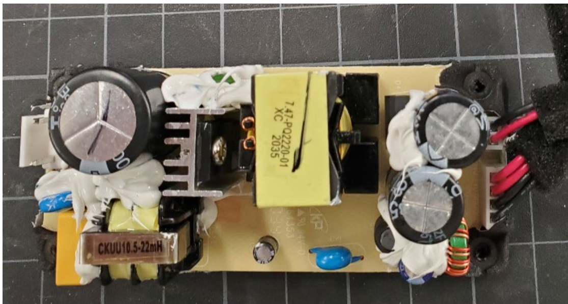
(fig. 5) AC/DC Power Supply (component side)
