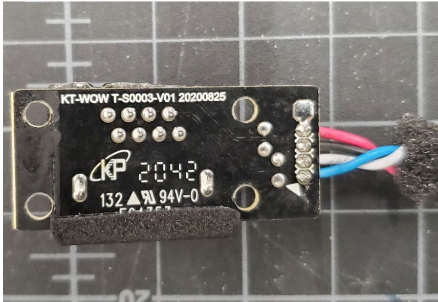
(fig. 3) RJ45 connector board (solder side)
