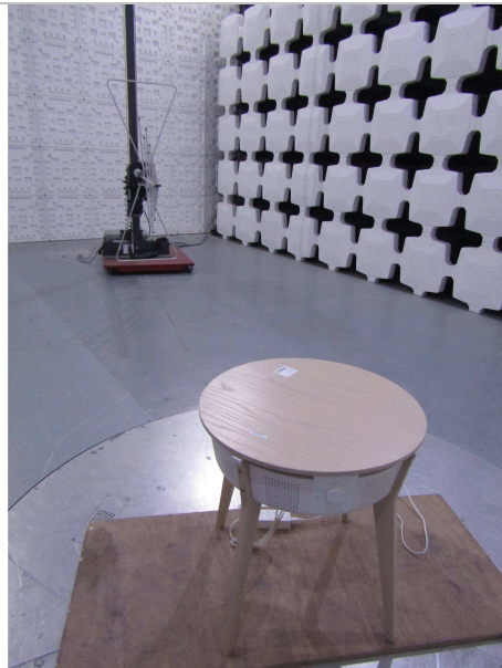
Radiated Emission (30 MHz–1000 MHz)
