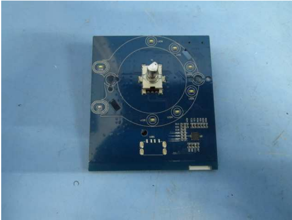
Main control board PCB view
