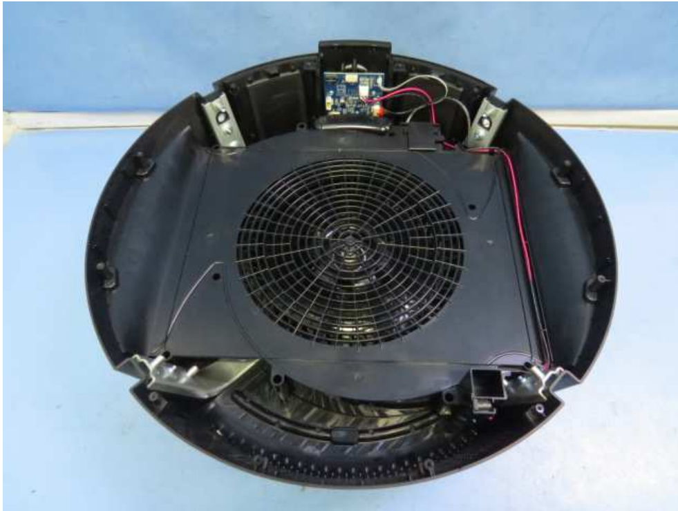
Inner view, location of main control board
