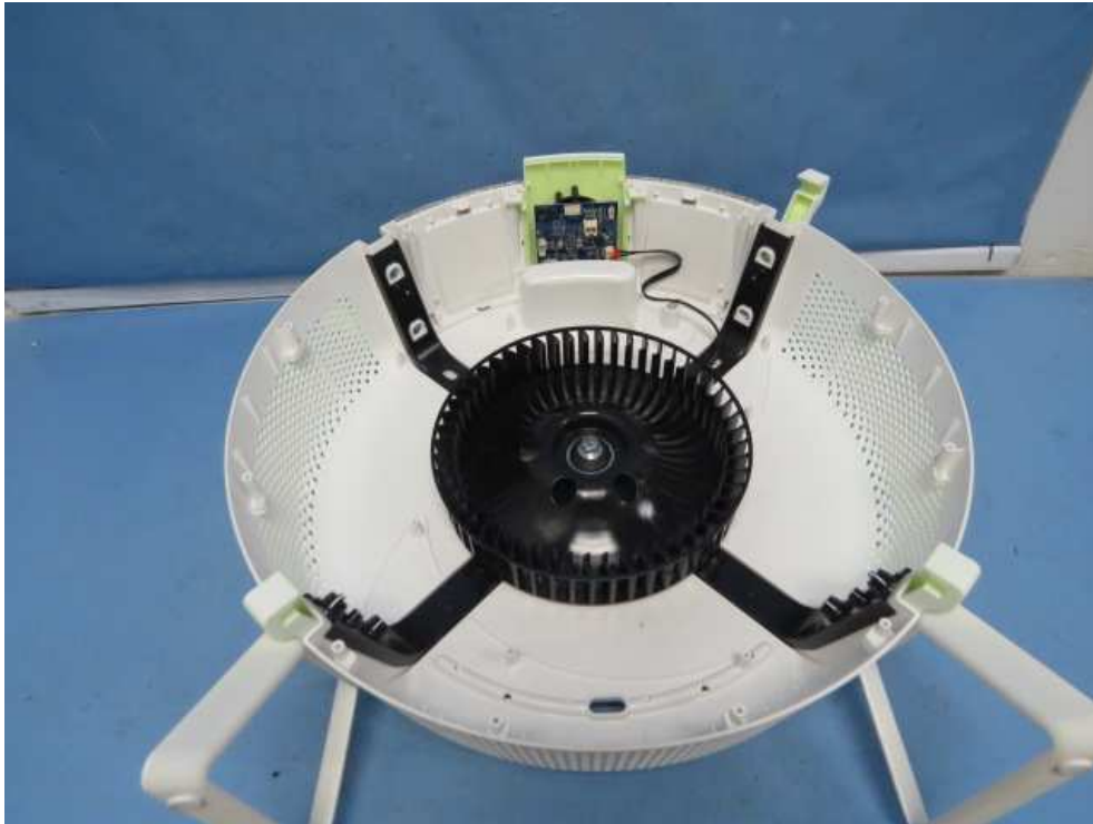
Inner view, location of fan motor
