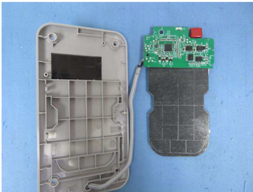
Internal view
