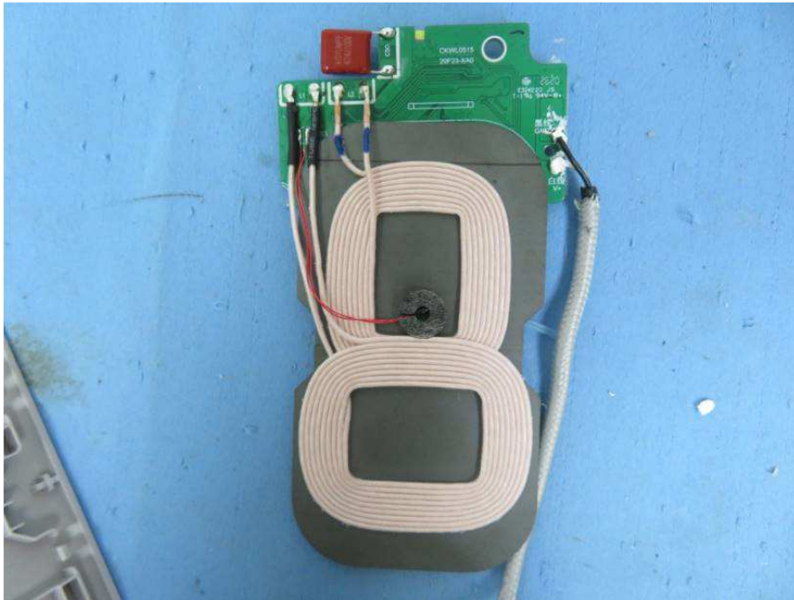
Internal view
