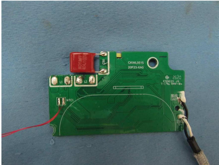
PCB view
