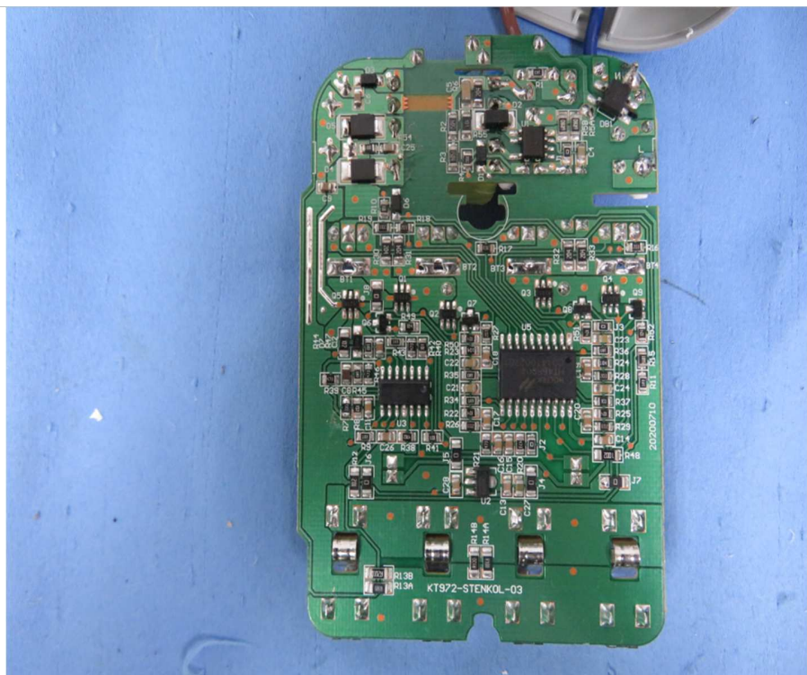
PCB view
