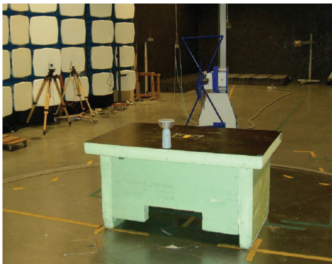
Test set up radiated emission 30 MHz – 1 GHz
