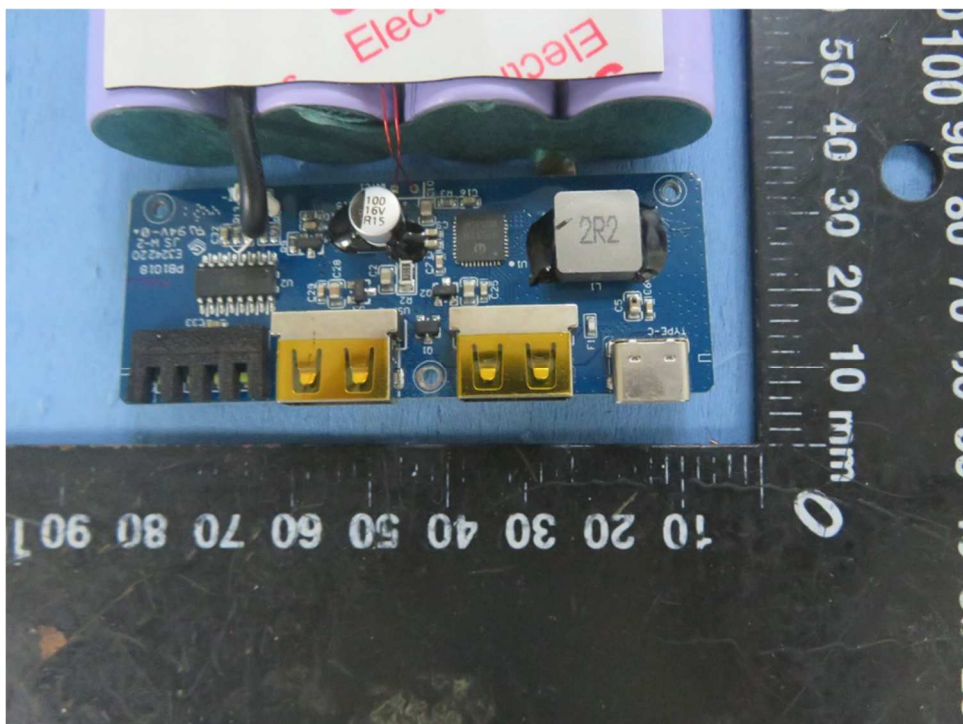
PCB view
