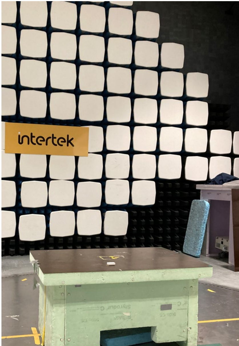
Photo(s) of test setup(s) for radiated disturbances 30 – 1000 MHz
