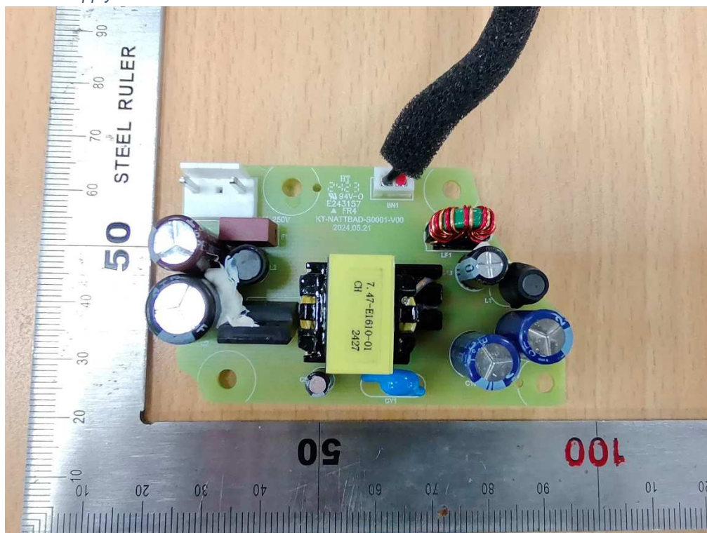
Bild / Picture 6: Power supply unit view
