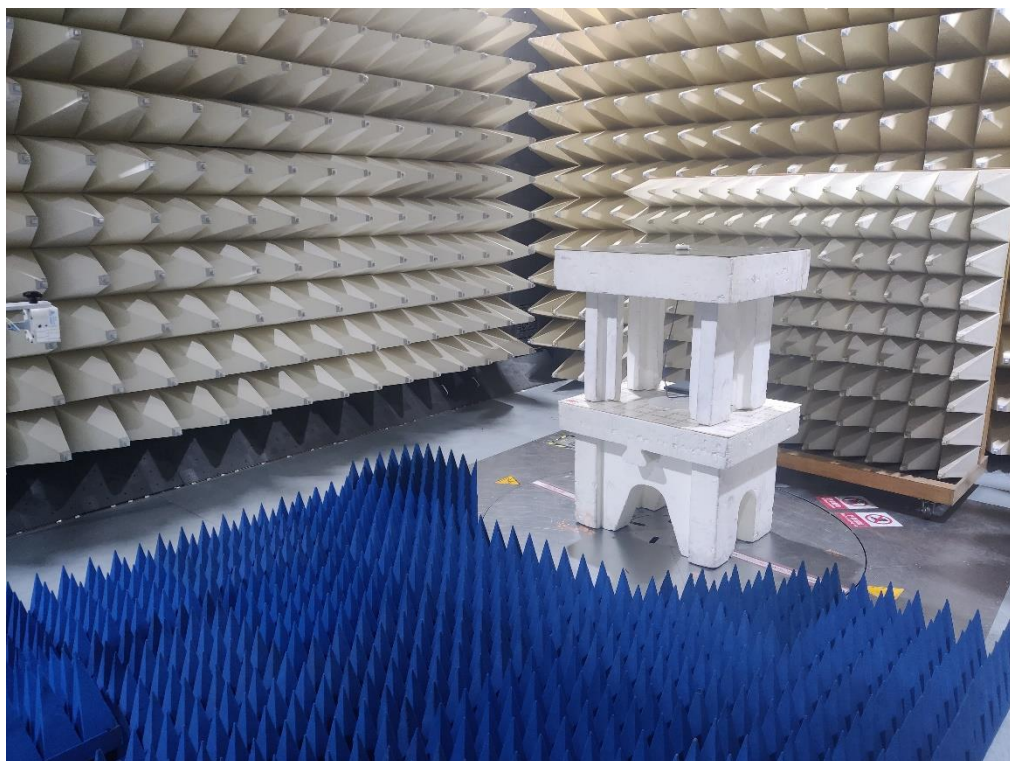
Photograph 4: Set-up photo for Radiated Emission, 18GHz - 25GHz
