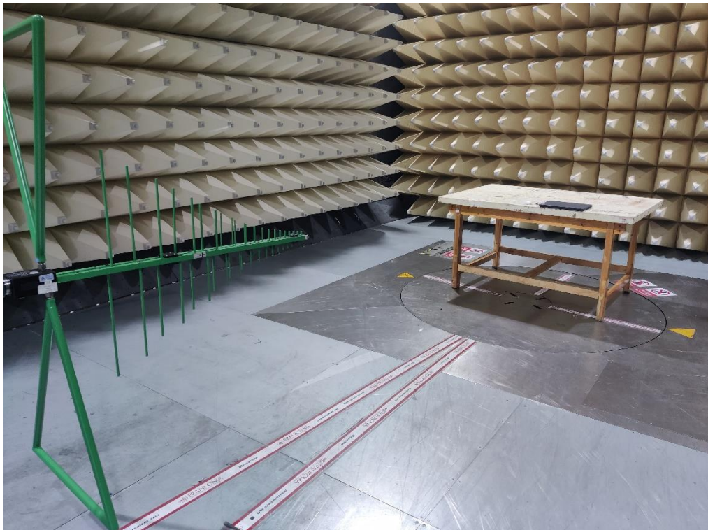
Photograph 2: Set-up photo for Radiated Emission, 30MHz - 1GHz
