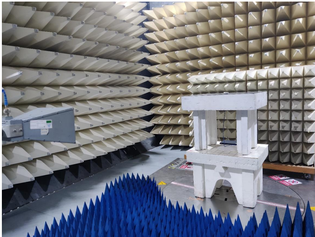
Photograph 3: Set-up photo for Radiated Emission, 1GHz - 18GHz
