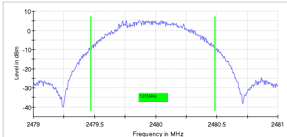
99 % Bandwidth
