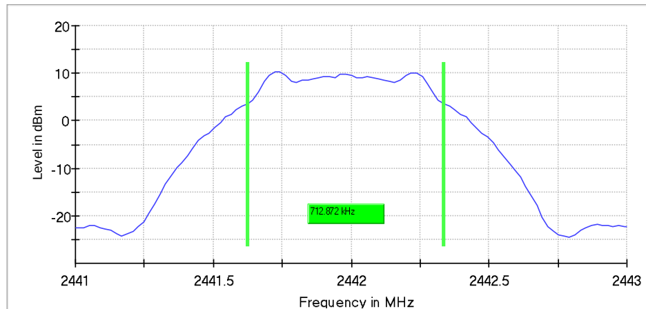
6 dB Bandwidth
