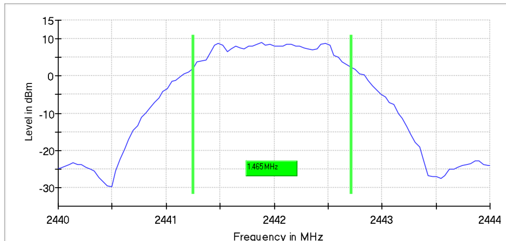
6 dB Bandwidth
