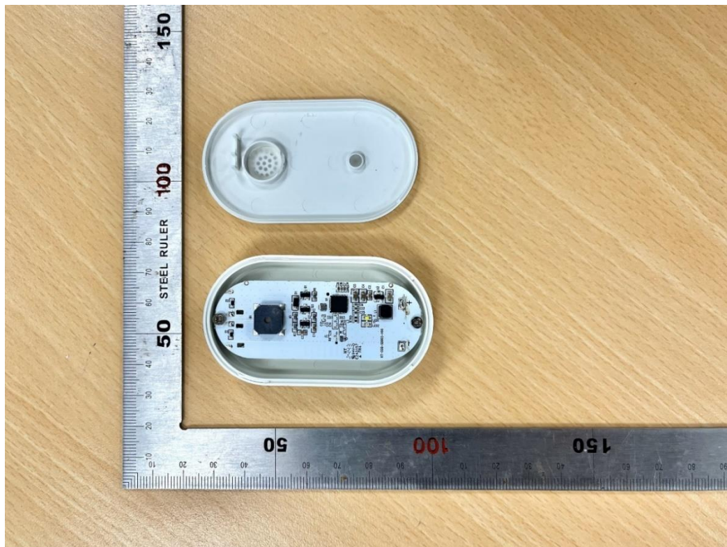
Bild / Picture 5: Internal view
