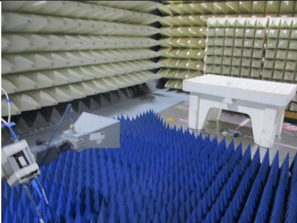
Above 1 GHz
