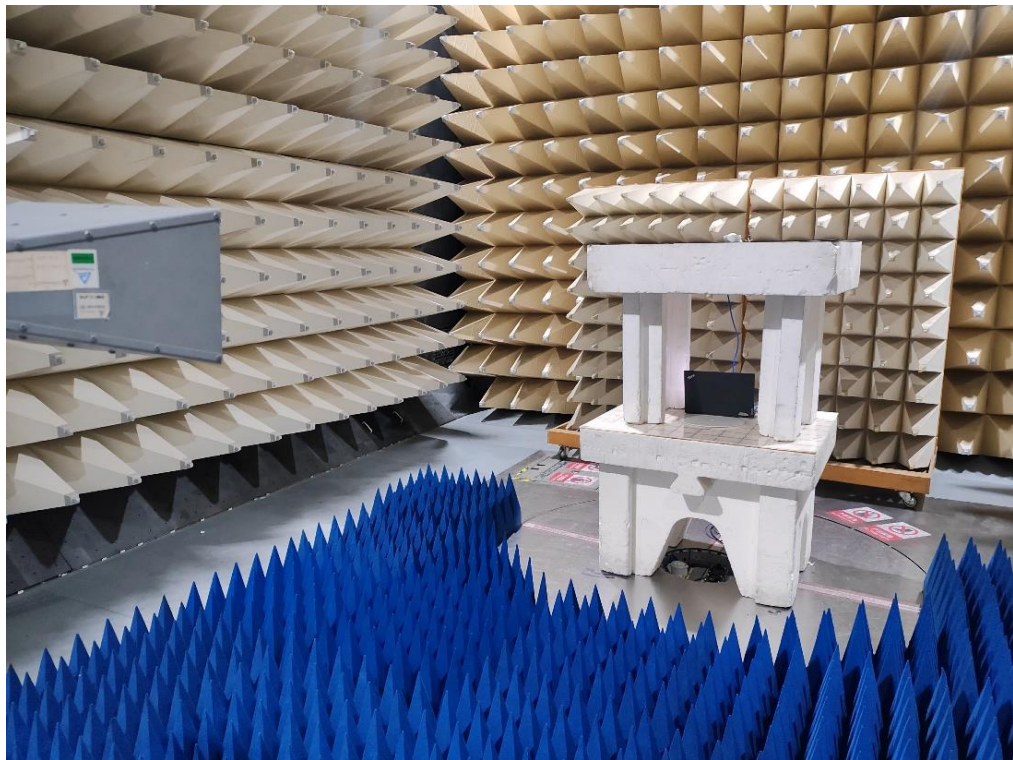
Photograph 3: Set-up photo for Radiated Emission, 1GHz - 18GHz
