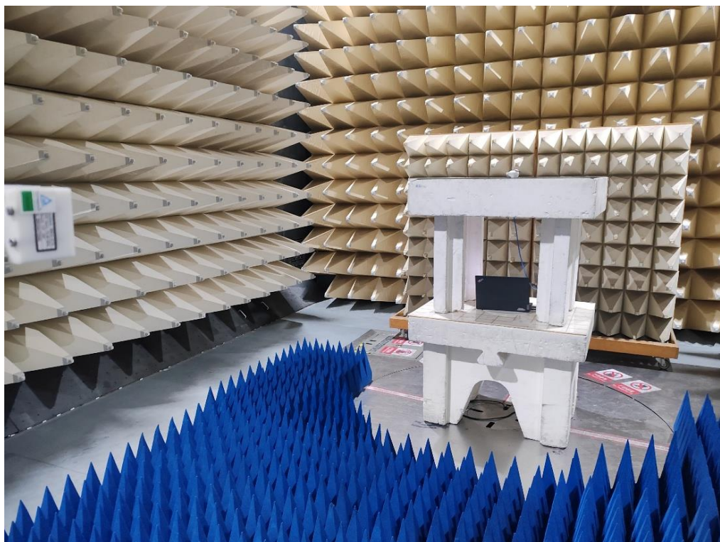
Photograph 4: Set-up photo for Radiated Emission, 18GHz - 25GHz
