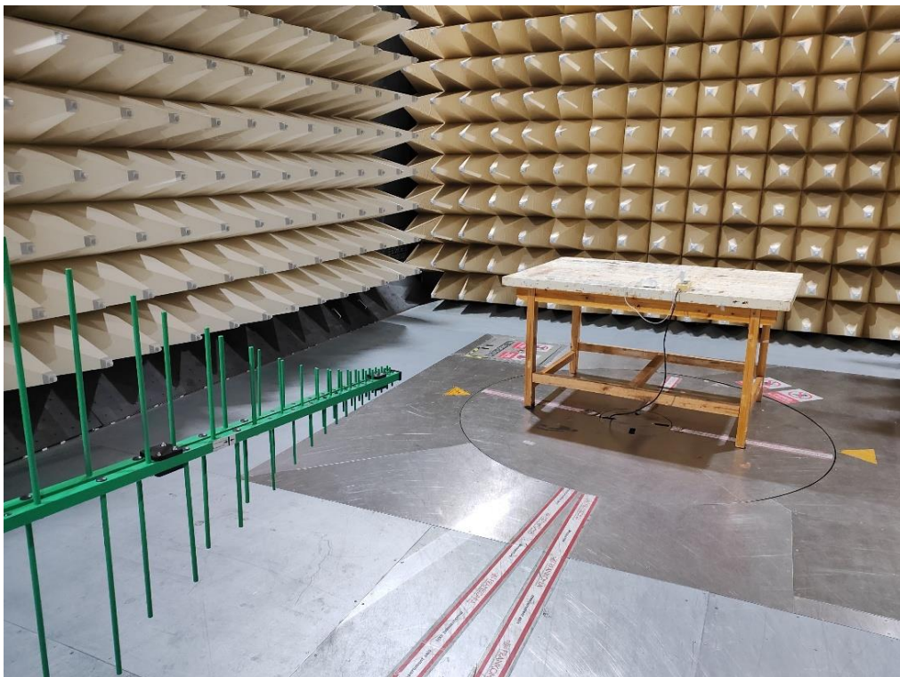
Photograph 3: Set-up for measurement of radiated emission
