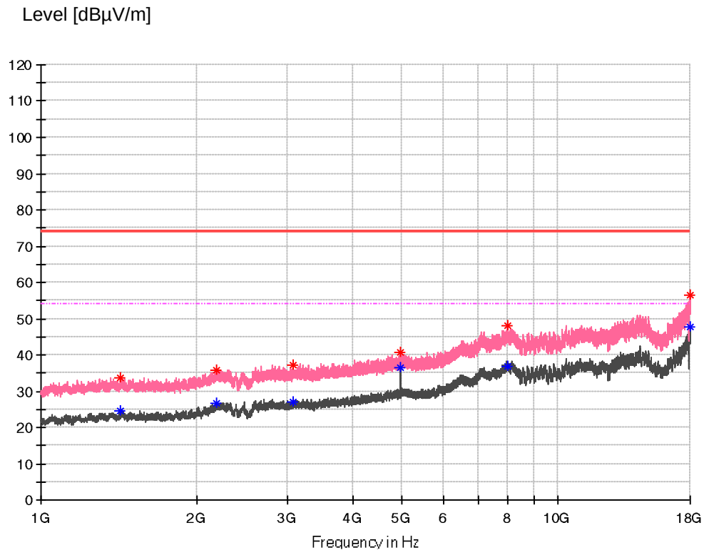
Figure 12: Spectral Diagrams and measurement results, 1 GHz – 18 GHz, Vertical polarization on mode 2
