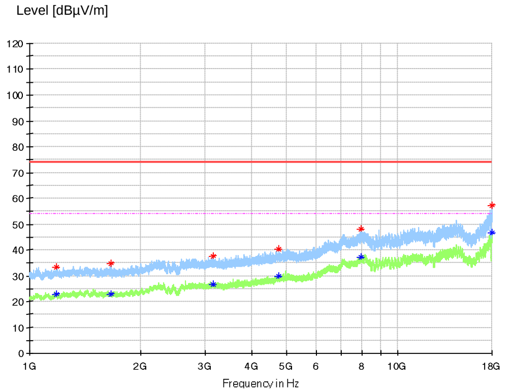
Figure 11: Spectral Diagrams and measurement results, 1 GHz – 18 GHz, Horizontal polarization on mode 2
