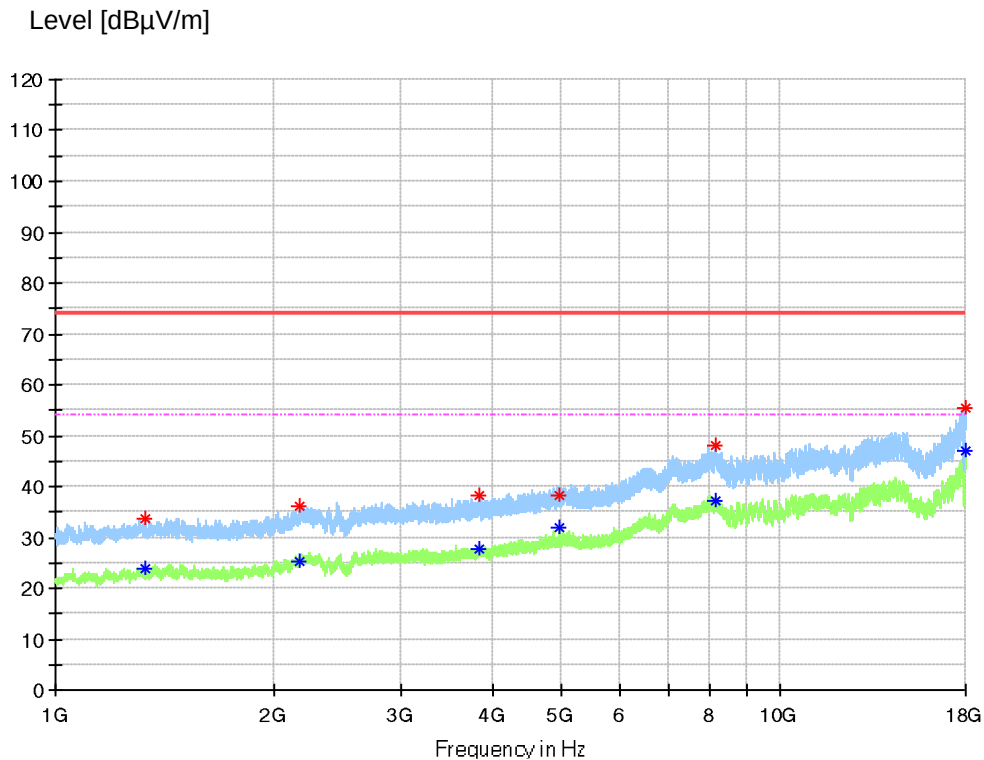
Figure 9: Spectral Diagrams and measurement results, 1 GHz – 18 GHz, Horizontal polarization on mode 1
