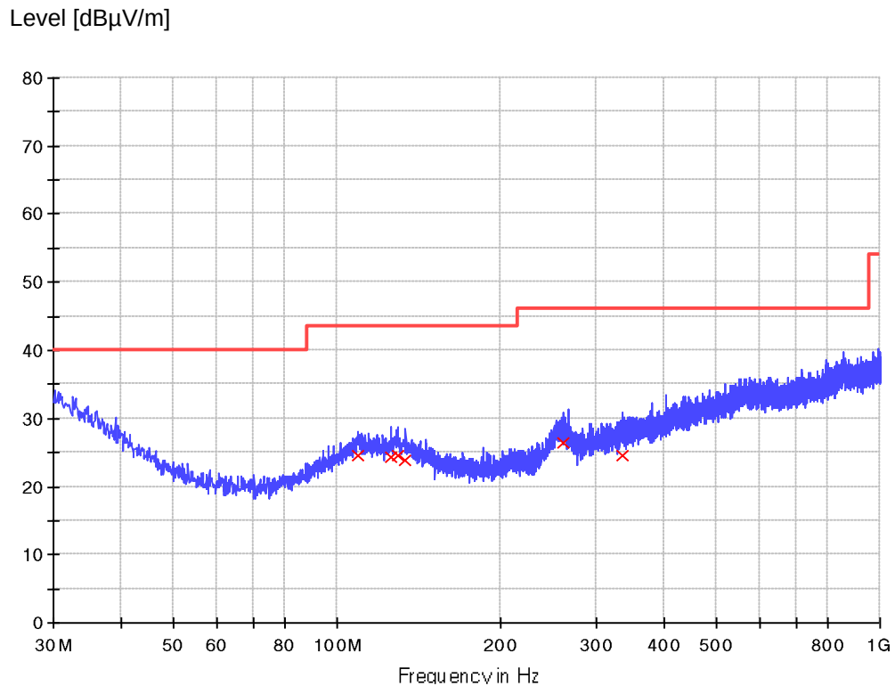
Figure 3: Spectral Diagrams and measurement results, horizontal polarization (30 MHz to 1 GHz)
