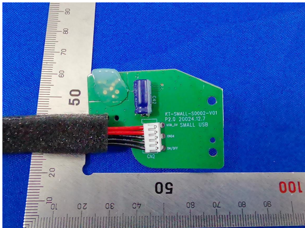
Bild / Picture 8: USB board view
