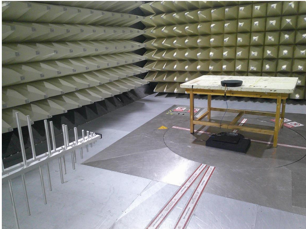
Photograph 3: Set-up photo for Radiated Emission, 30MHz - 1GHz
