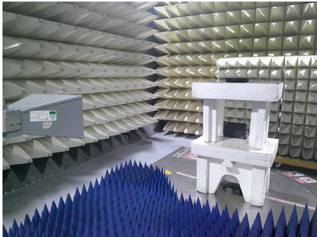
Photograph 4: Set-up photo for Radiated Emission, 1GHz - 18GHz
