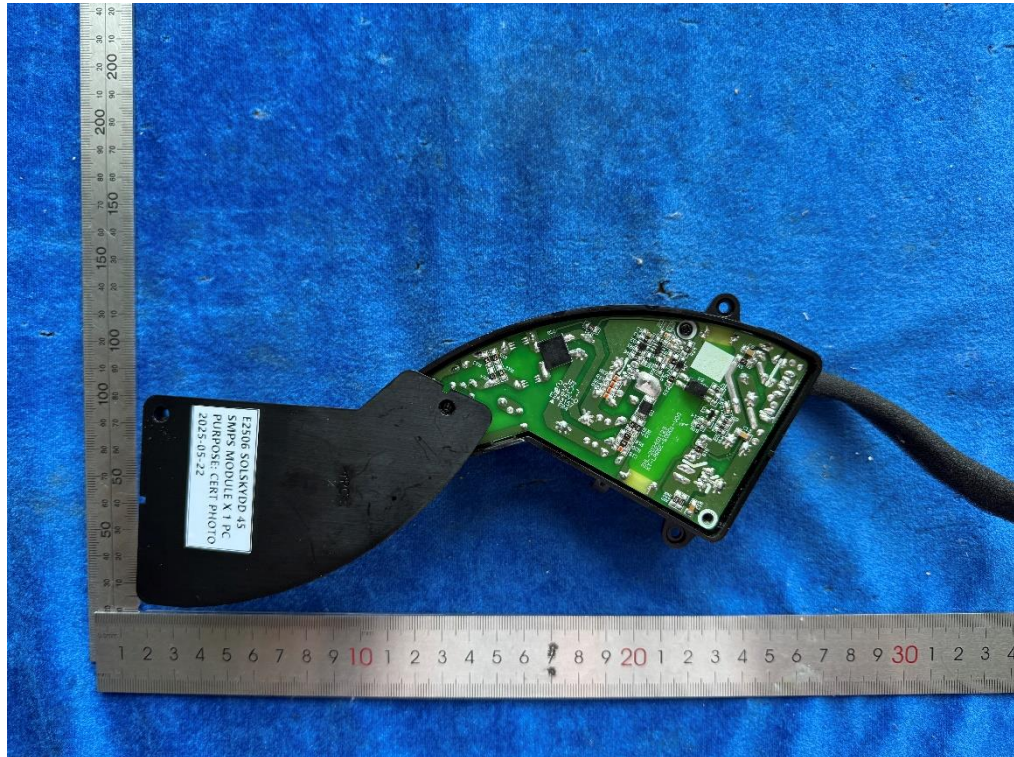
Bild / Picture 5: Internal view of power board unit
