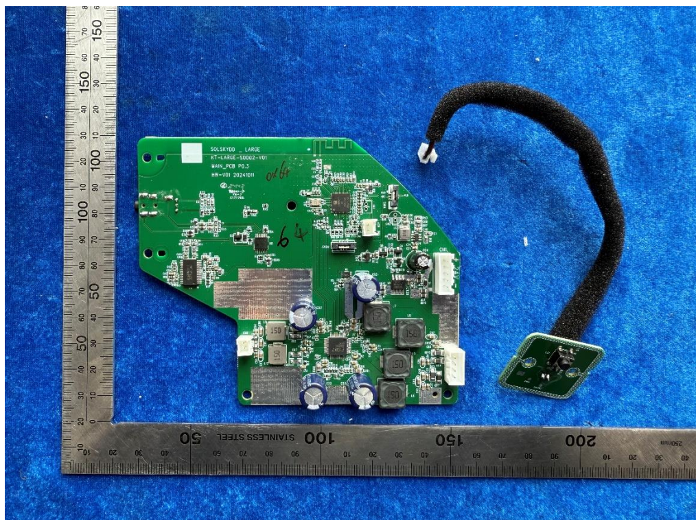
Bild / Picture 6: Internal view of main board
