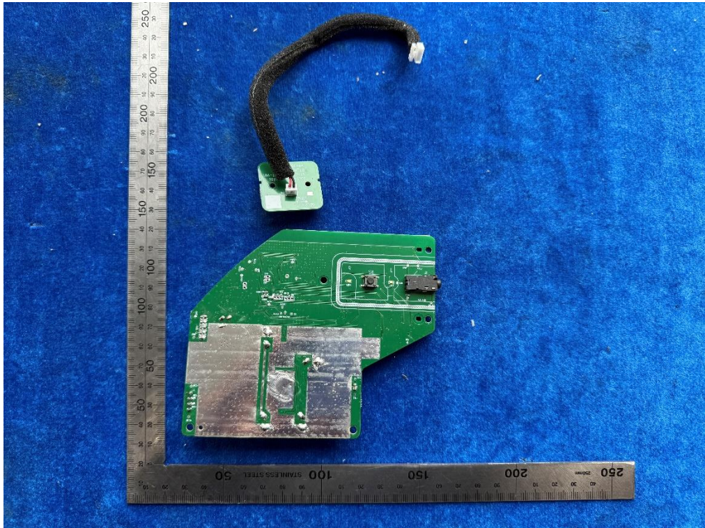
Bild / Picture 8: Woofer view
