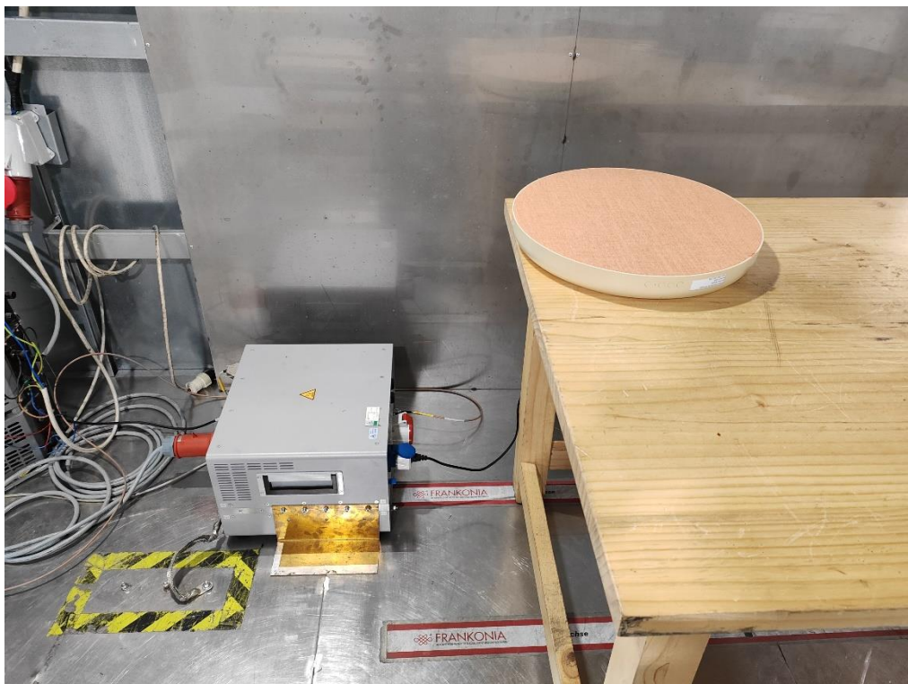
Photograph 2: Set-up for measurement of conducted emission
