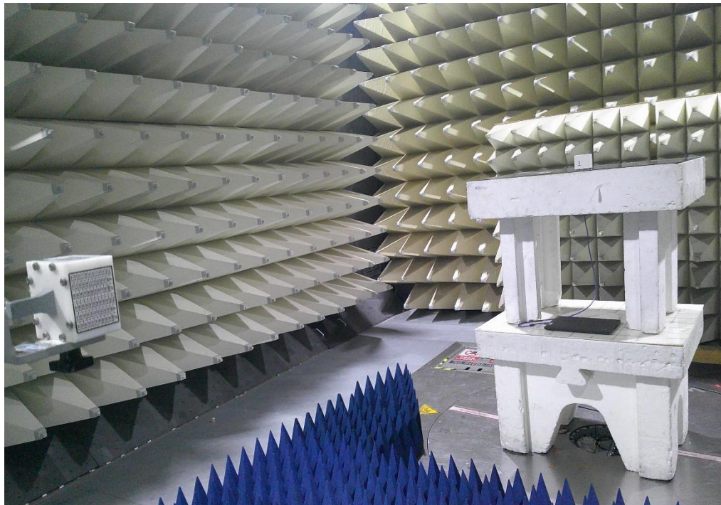
Photograph 5: Set-up photo for Radiated Emission, 18GHz - 25GHz
