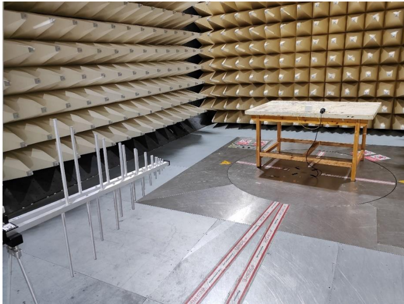
Photograph 3: Set-up for measurement of radiated emission
