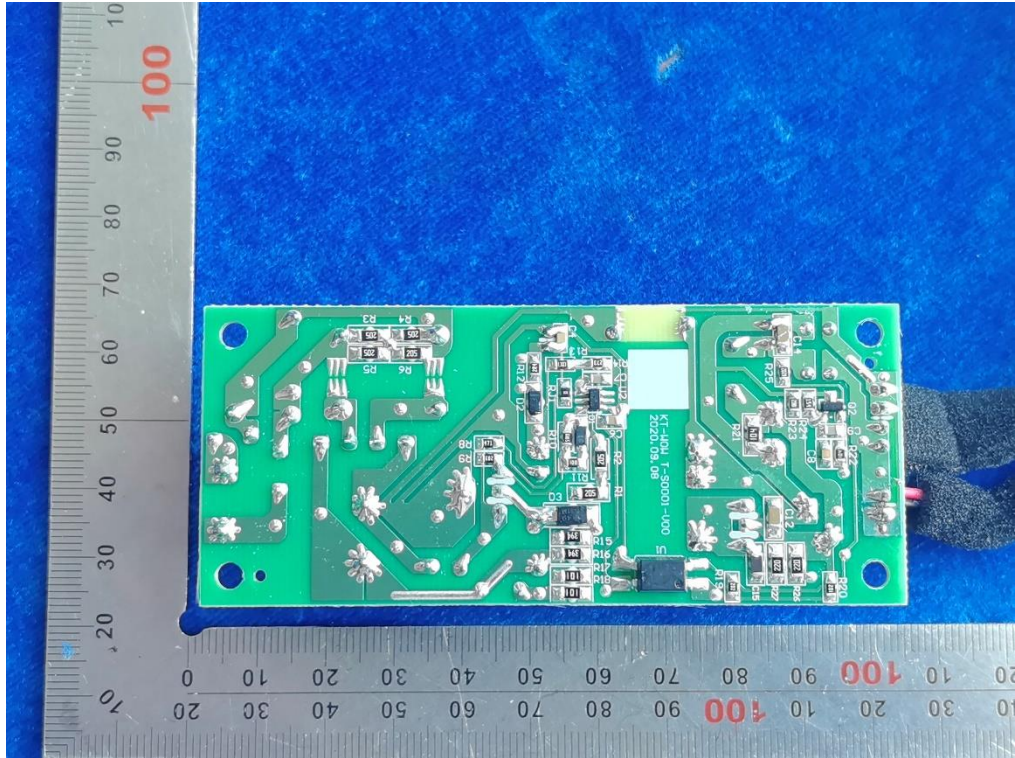
Bild / Picture 17: Power supply unit view
