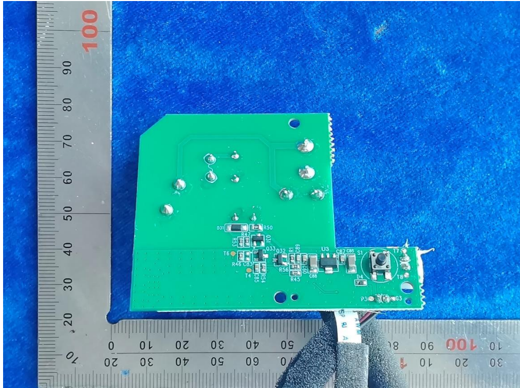
Bild / Picture 16: Power supply unit view
