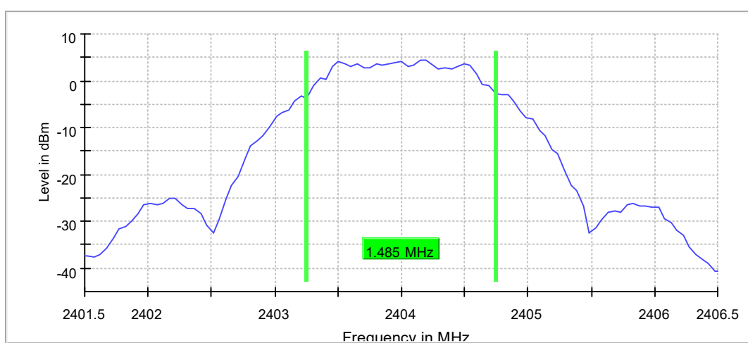
6 dB Bandwidth
