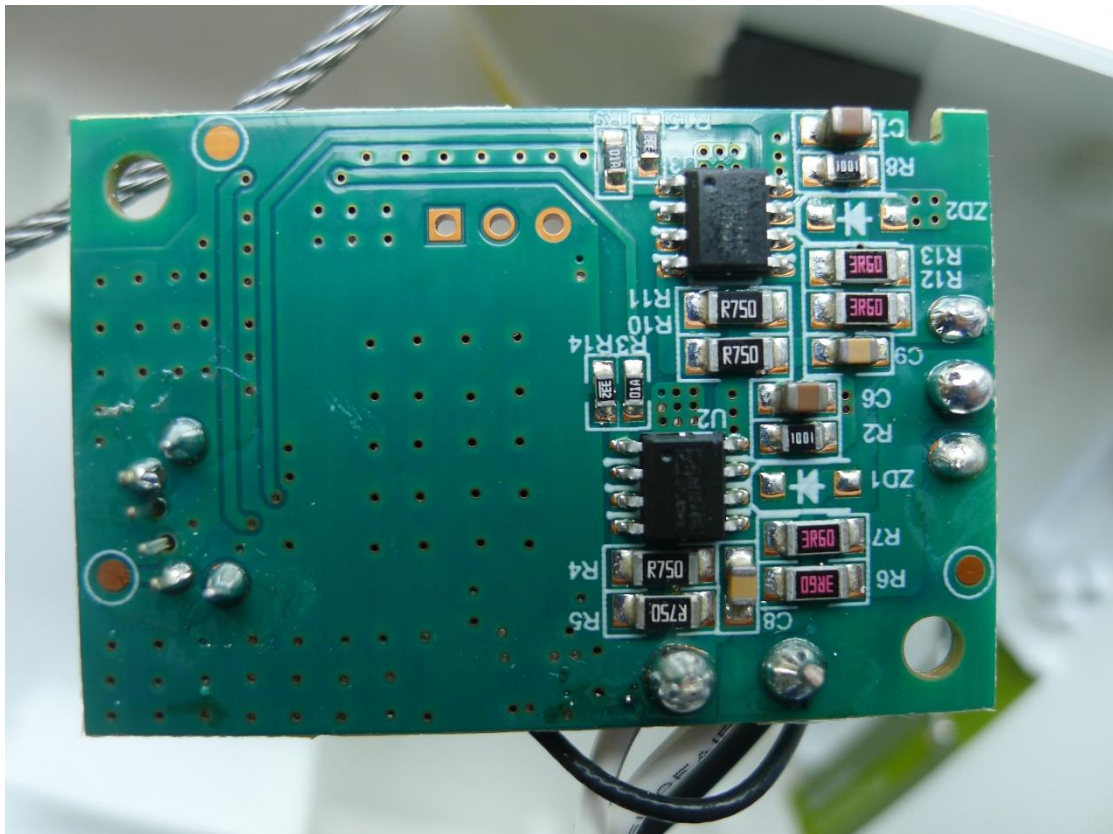
Electronic Circuit
