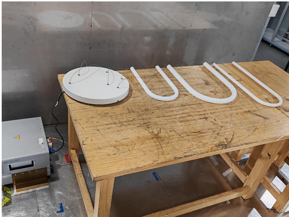
Photograph 2: Set-up photo for Conducted Emission
