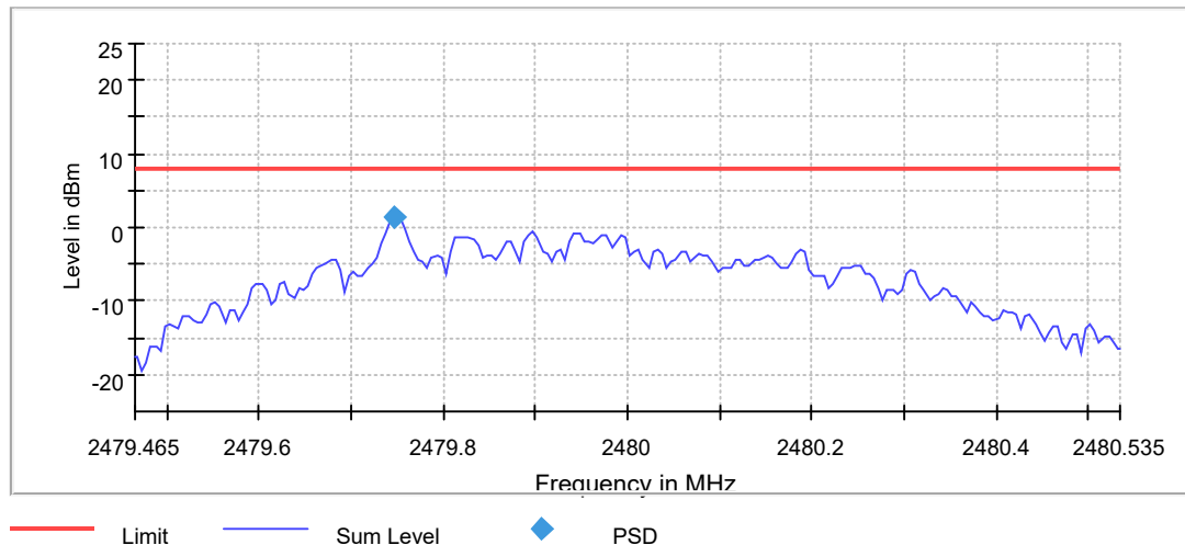
Peak Power Spectral Density(2)
