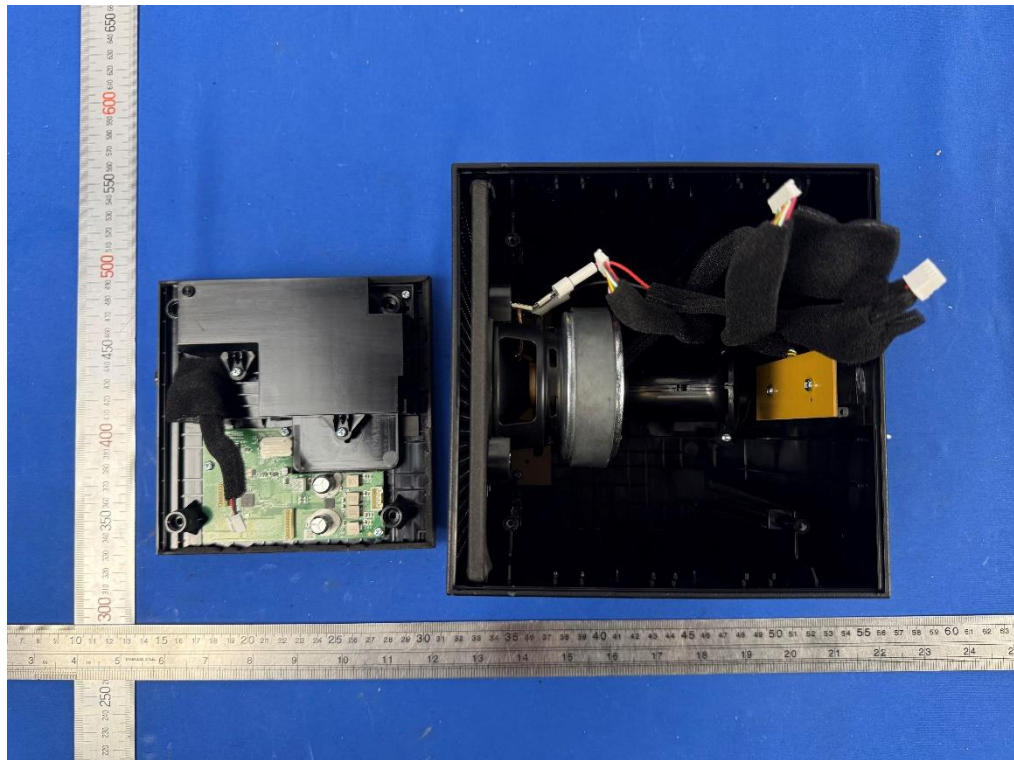
Bild / Picture 2: Internal view of Speakers
