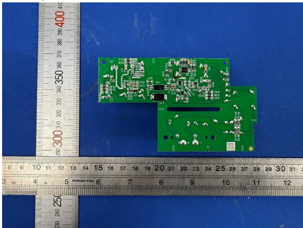
Bild / Picture 8: Internal view of main board
