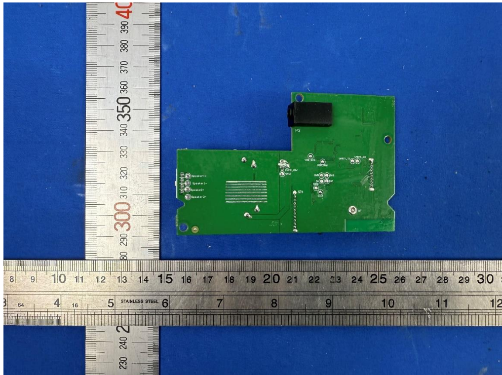
Bild / Picture 9: Internal view of main board
