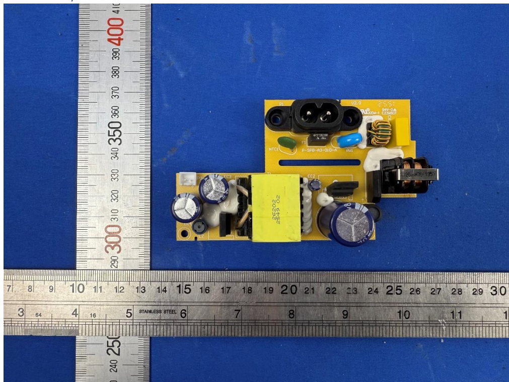
Bild / Picture 6: View of the power board
