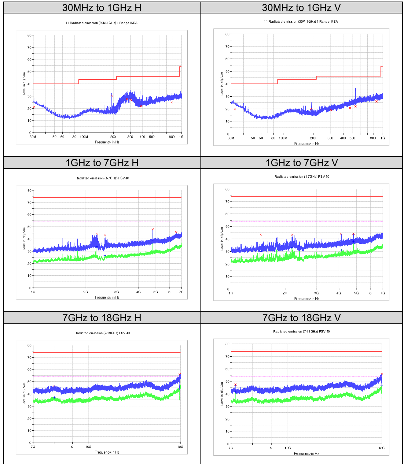
Figure 10: Radiated Spurious Emission, 2402MHz
