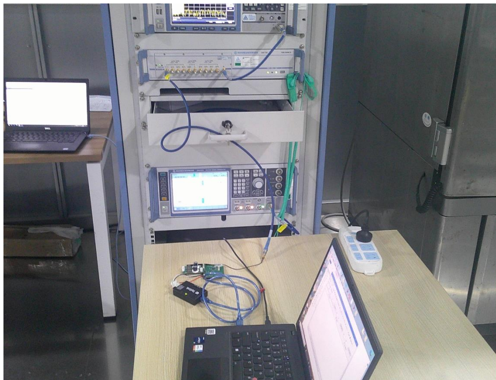
Photograph 1: Set-up photo for RF Conducted Test
