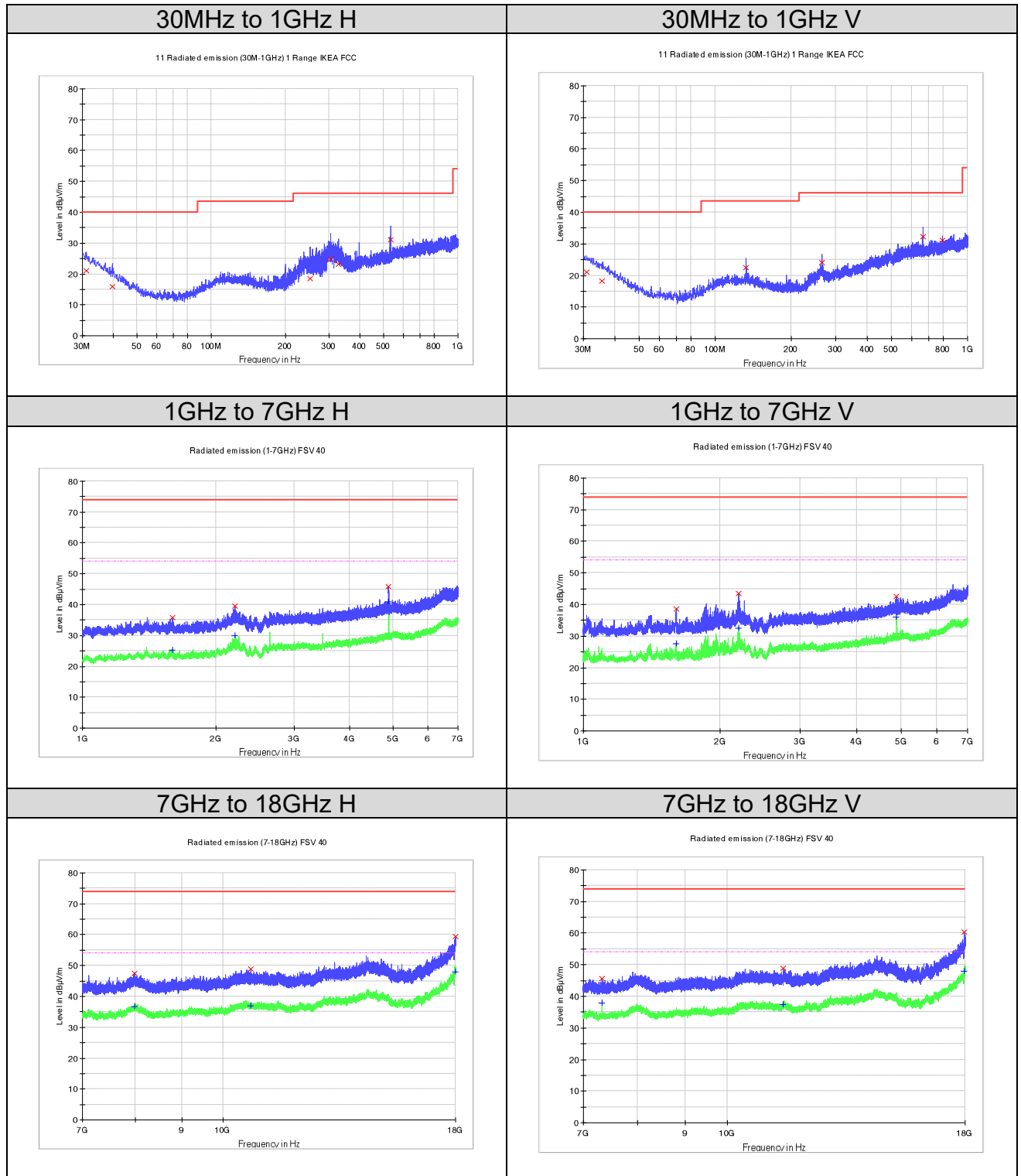
Figure 9: Radiated Spurious Emission, 2445MHz
