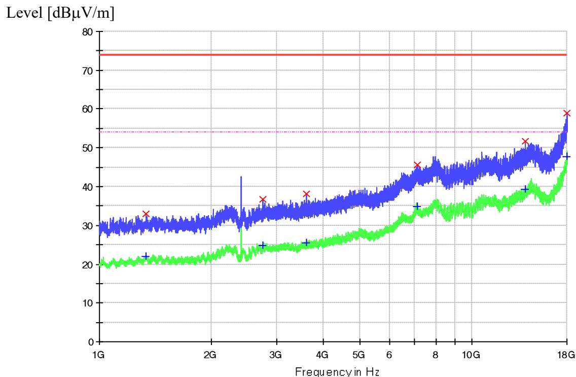
Figure 4: Spectral Diagrams and measurement results, 1-18 GHz, vertical polarization
