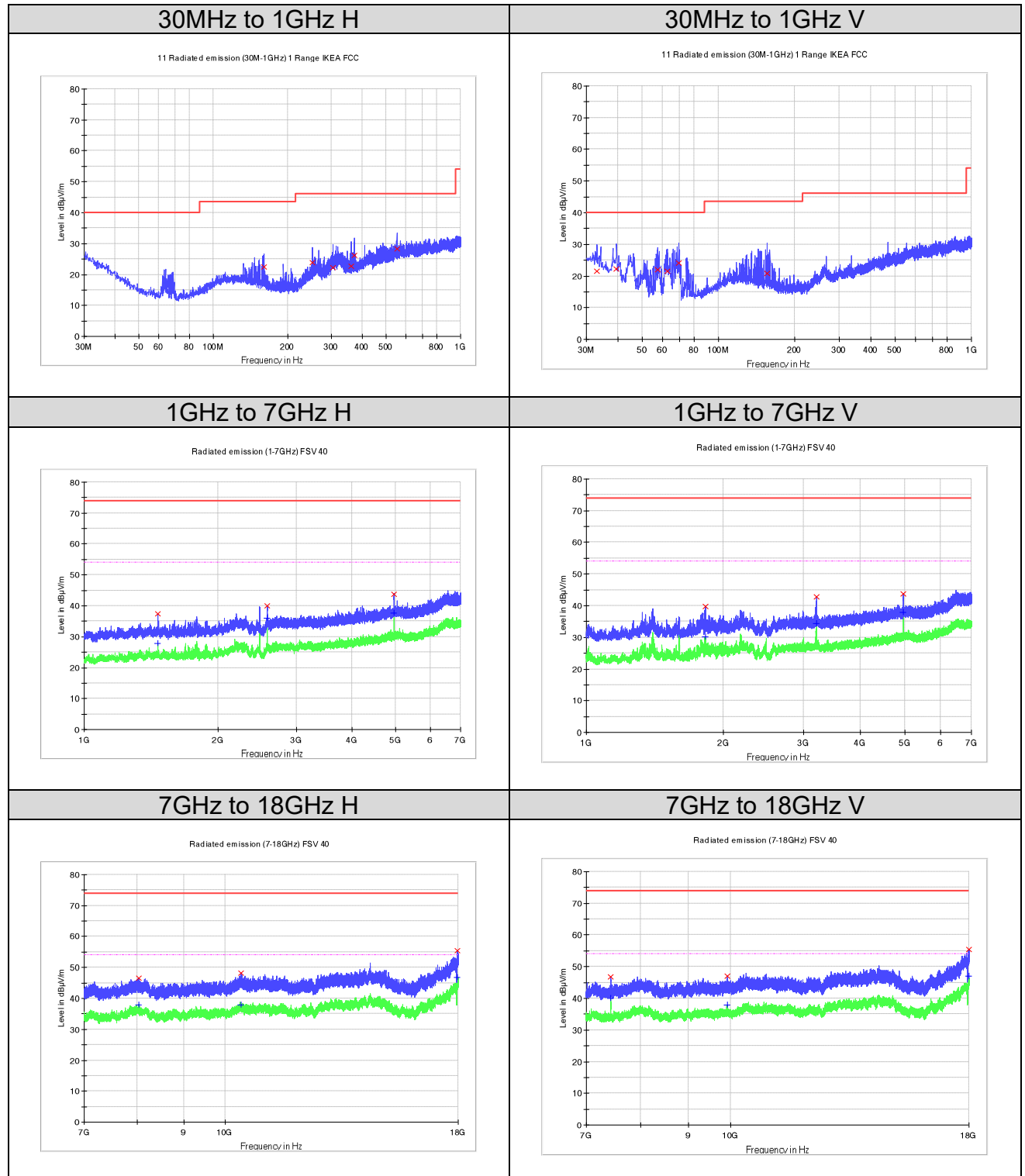
Figure 14: Radiated Spurious Emission, 2Mbps, 2478MHz
