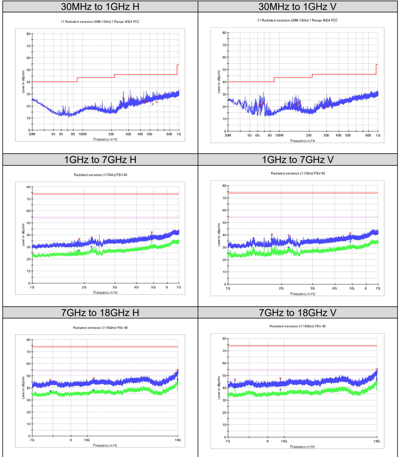
Figure 13: Radiated Spurious Emission, 2Mbps, 2440MHz
