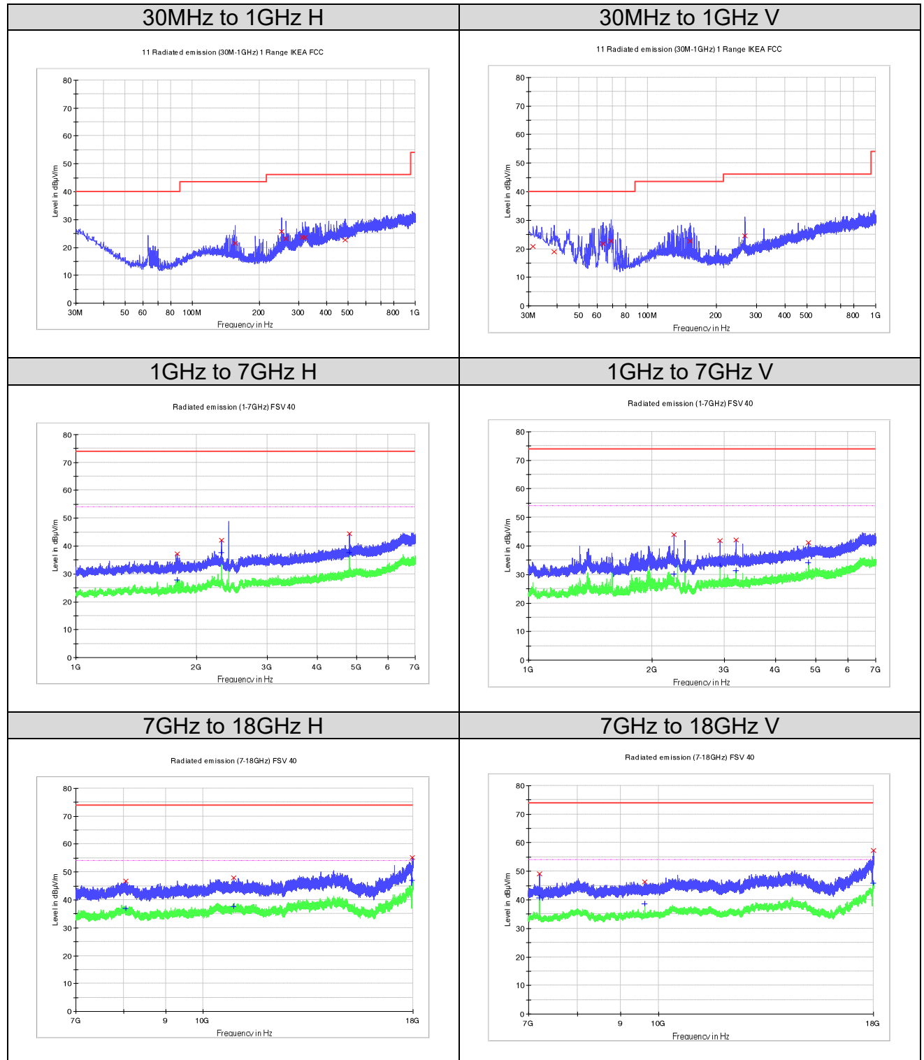
Figure 12: Radiated Spurious Emission, 2Mbps, 2404MHz
