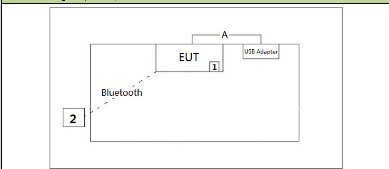
Connection Diagram (Mode 2)
