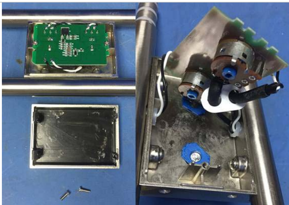
Internal view
