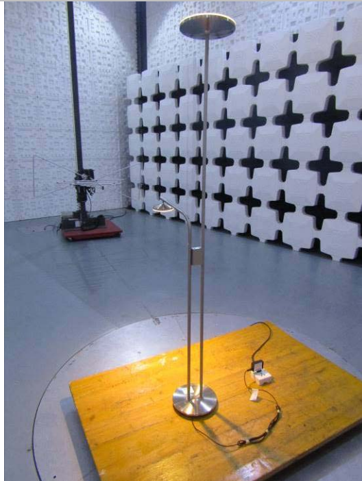
Radiated Emission (30 MHz–1000 MHz)
