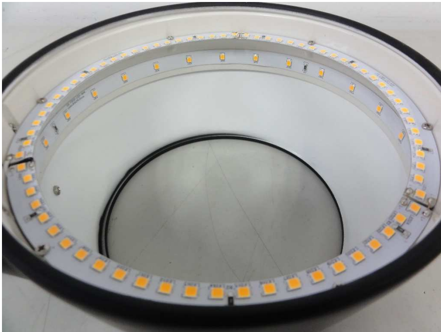
LED module
