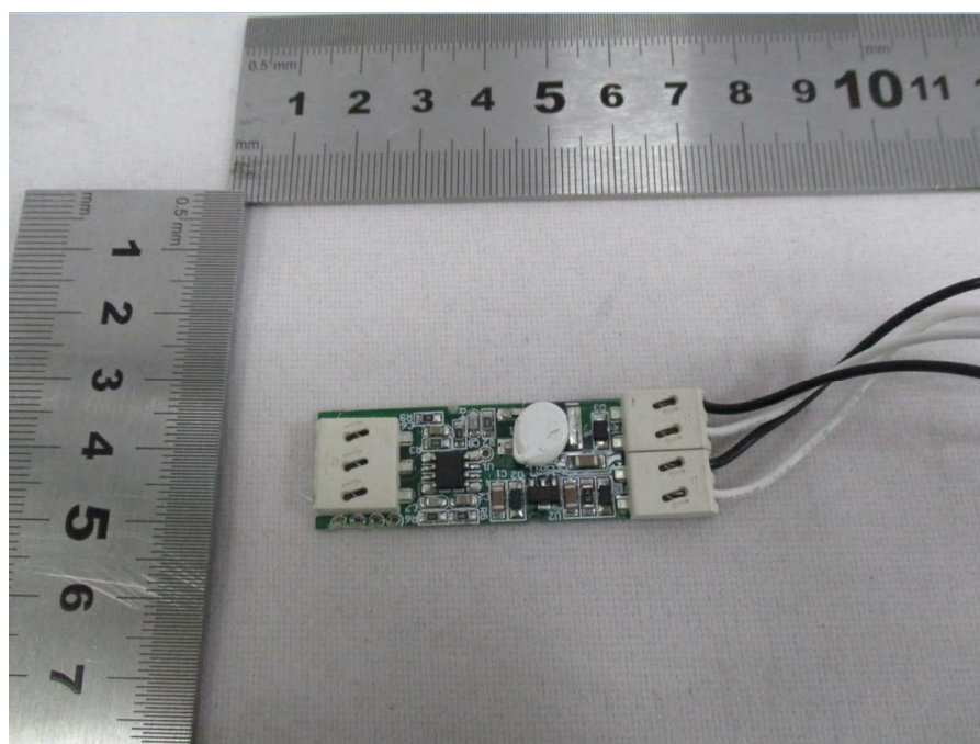
Dimmer PCB
