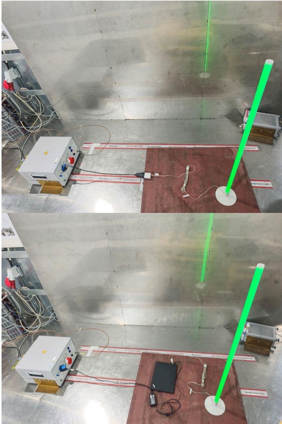
Photograph 1: Set-up for measurement of conducted emission
