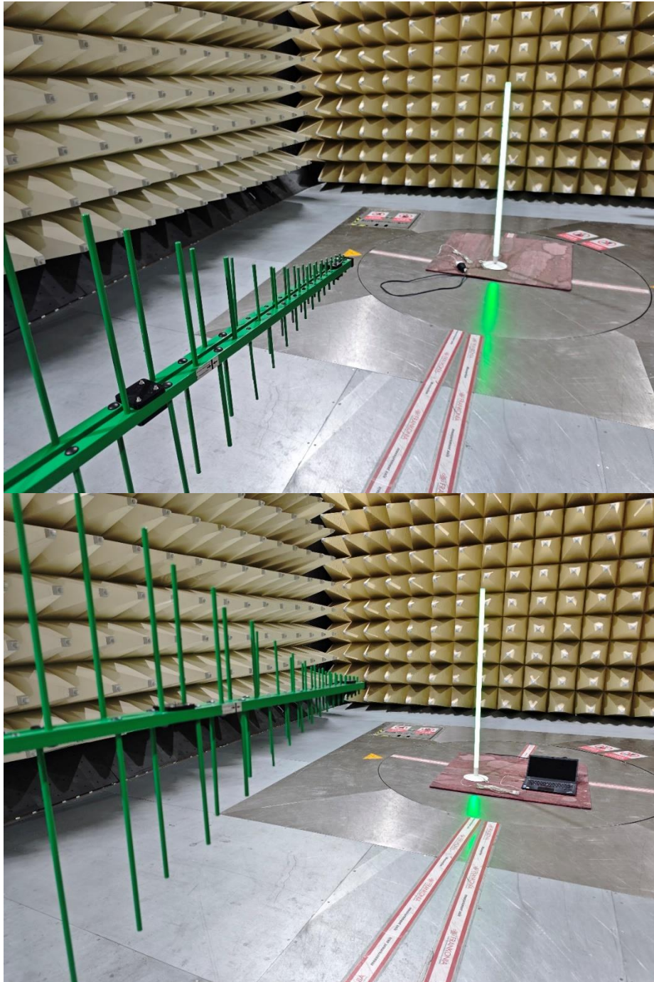
Photograph 2: Set-up for measurement of radiated emission
