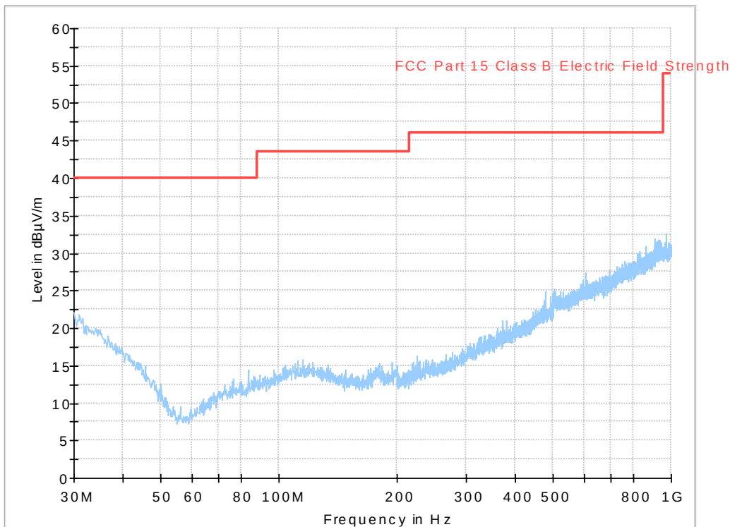
Diagram, Peak overview sweep, 30 – 1000 MHz at 3 m distance. RX middle channel, EUT orientation X.
