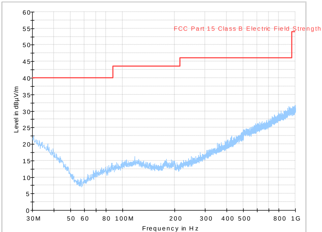
Diagram, Peak overview sweep, 30 – 1000 MHz at 3 m distance. RX low channel, EUT orientation Z.
