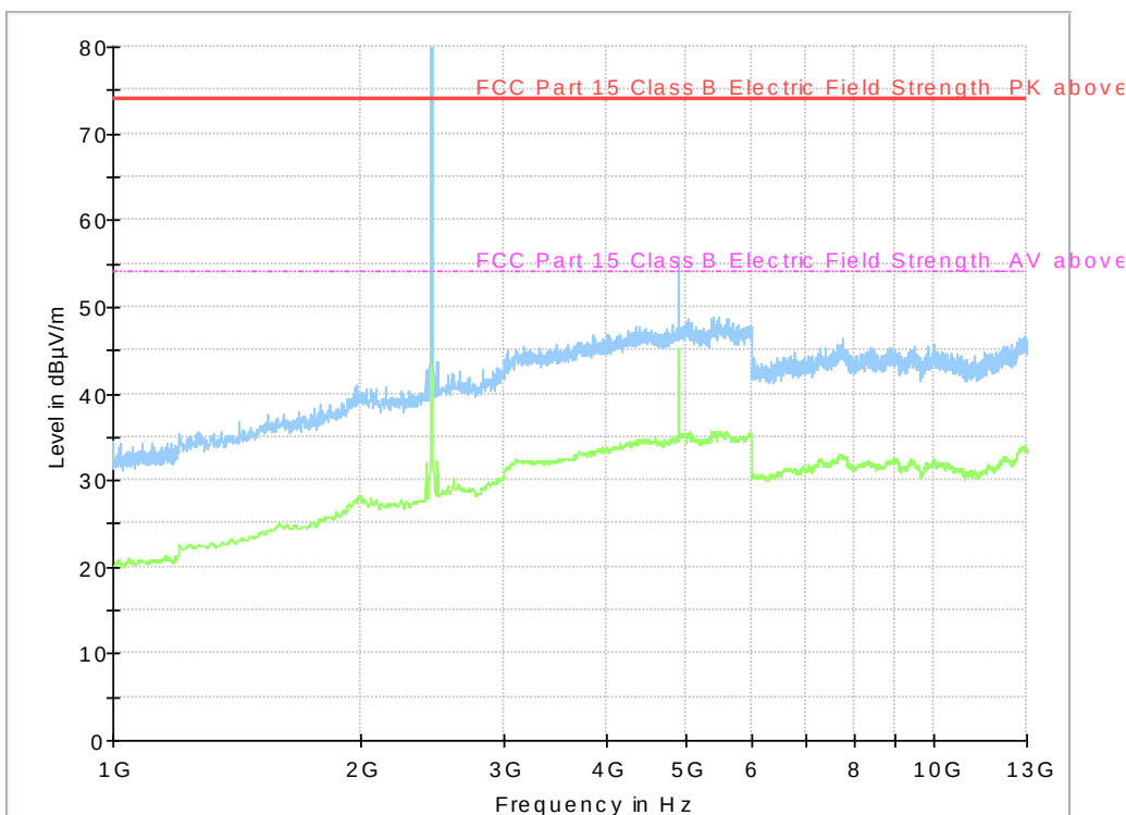
Diagram, Peak overview sweep, 1 – 13 GHz at 3 m distance. TX middle channel, EUT orientation Y.
