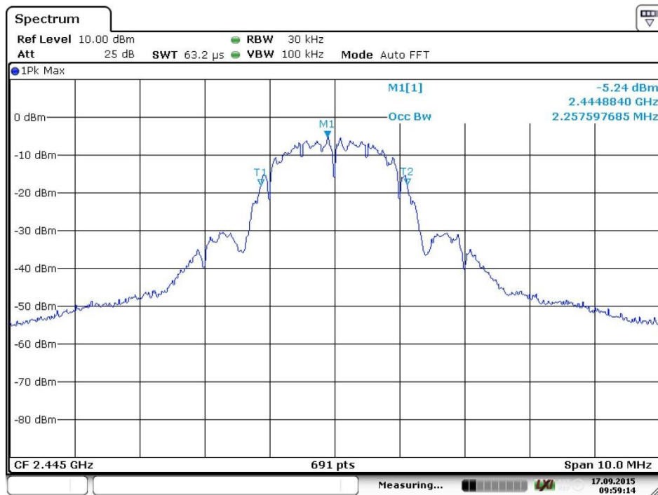
Screenshot: Occupied bandwidth Measurement, middle channel
