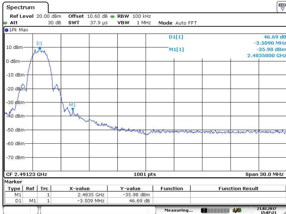
Screenshot: Upper band edge sweep, single channel
