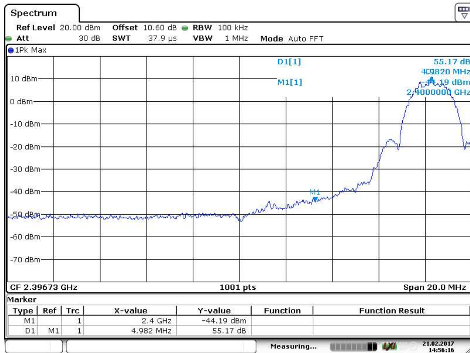
Screenshot: Lower band edge sweep, single channel
