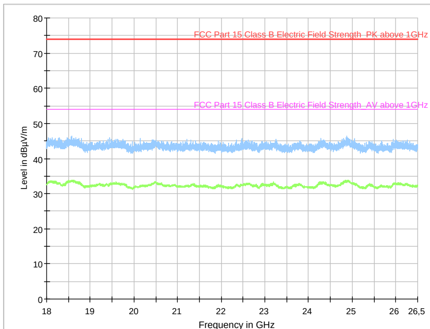
Diagram, Peak overview sweep, 18 – 26 GHz at 3 m distance. TX middle channel
