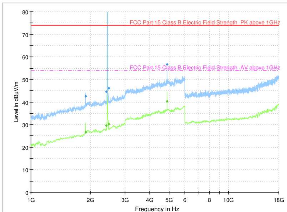
Diagram, Peak overview sweep, 1– 18 GHz at 3 m distance. TX middle channel
